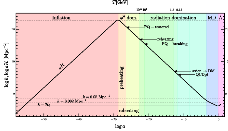
Figure 2: The history of the Universe in SMASH HHSI, emphasising the transition from inflation to radiation-domination-like Universe expansion aH \propto 1/a before standard matter and cosmological constant domination epochs [11].
