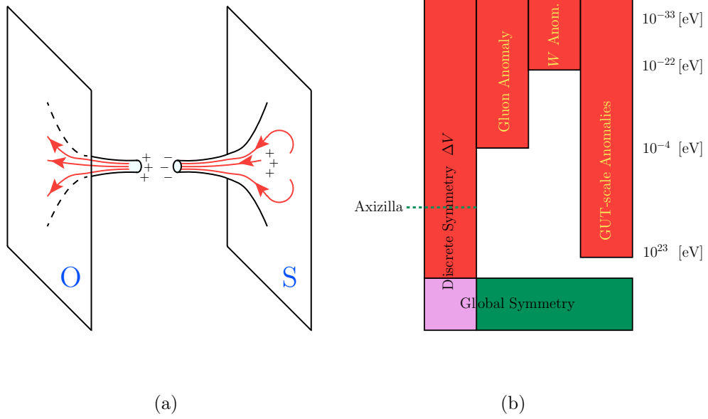
Figure 2: (a) A wormhole connecting our world to a shadow world, and (b) terms allowed by discrete and global symmetries.
