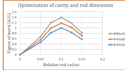
Figure 4: Figure of merit vs. relative rod radius at \epsilon_r=9 for various cavity dimensions.
