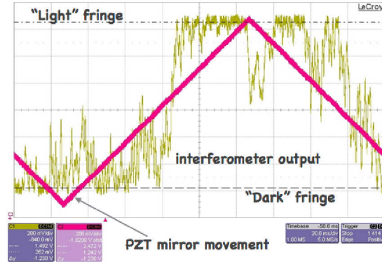
Figure 3: Sample oscilloscope screenshot illustrating interferometer calibration. The yellow trace is the photodiode signal, while the red trace is the voltage ramp applied to the piezo-actuated mirror (see also text).
