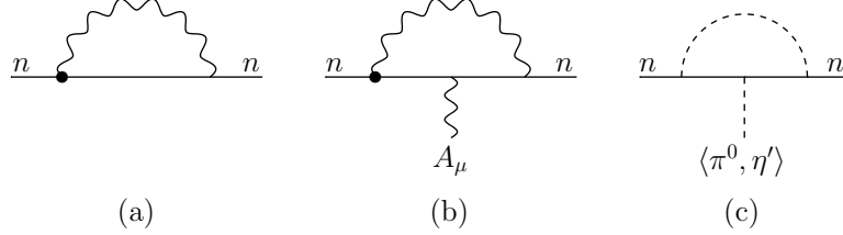
Figure 1: The bullets in (a,b) are the insertions of CP violating interaction shown in (c). VEVs of \pi^0 and \eta' break CP. (b) leads to nEDM.
