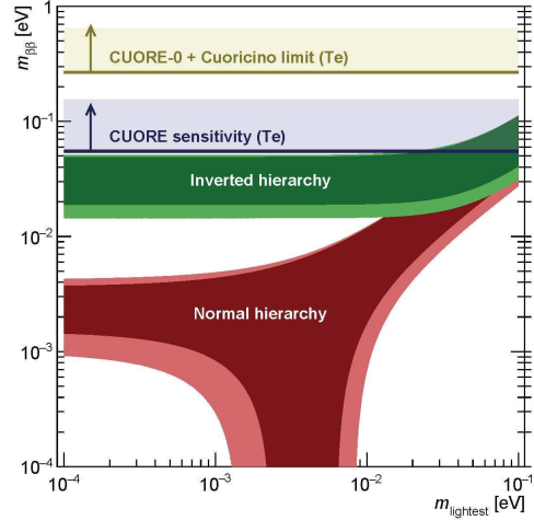
Figure 2: Allowed regions for the effective Majorana neutrino mass for the normal and inverted hierarchies, CUORE-0+Cuoricino 90% limit and expected CUORE 90% sensitivity (5 years live time).
