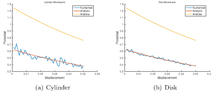
Figure 2: Monte-Carlo Calculation
