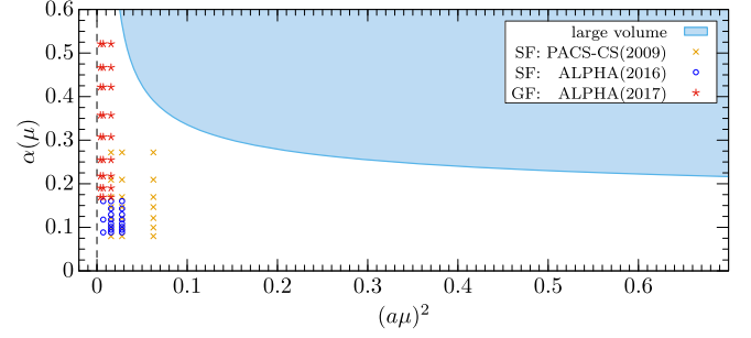
FIG. 1. The shaded area shows the a > 0.04 \text{ fm} region of large volume results which dominate the present PDG and FLAG estimates [7,17] of \alpha_{\text{MS}}(\mu) . The boundary of the shaded area is determined by \alpha_{\text{MS}}(\mu) evaluated at two-loop order for N_f = 3 and \Lambda_{\text{MS}}^{(3)} = 341 \text{ MeV} . The x coordinate is then obtained by setting a = 0.04 \text{ fm} , the smallest value of lattice spacings reached in the large volume simulations entering [7,17]. The data points on the left are finite-size scaling computations [8,13,14].
