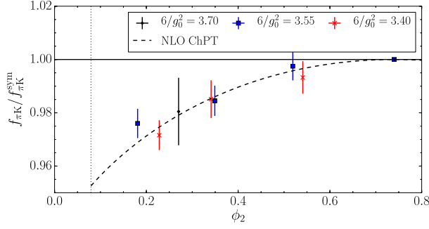
FIG. 3. Dependence of f_{\pi K} at \phi_4 = 1.11 on the pion mass through \phi_2 = m_\pi^2/\mu_{\text{ref}}^2 [31]. We normalized to f_{\pi K}^{\text{sym}} at the symmetric point m_u = m_d = m_s . The ratio follows the parameter-free prediction of NLO chiral PT.
