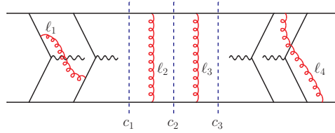
Fig. 6. Graph for double Drell-Yan production with several soft gluons exchanged between left and right moving fast partons. The three possible final state cuts of the graph are denoted by c_1, c_2 and c_3 .
