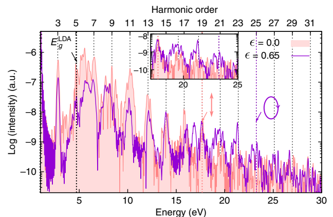
Fig. 5 Ellipticity-based HHG cutoff extension. Computed HHG spectra from bulk MgO for linearly polarized and elliptically polarized ( \epsilon = 0.65 ) driving pulses. In both cases, the major axis of the polarization ellipse along the \overline{\Gamma K} . The dashed lines indicate the position of the cutoff energy ( E_c ). The inset shows a zoom into the spectral region around the extended energy cutoff
