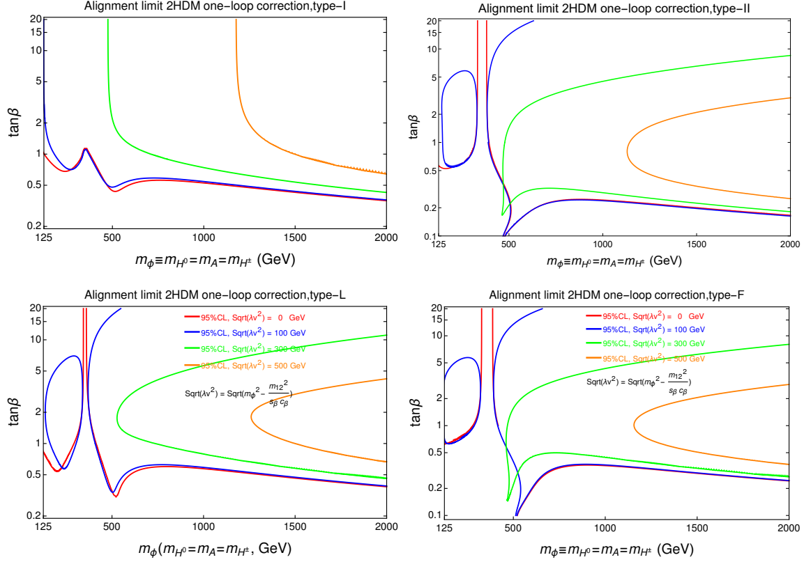
Figure 6. 95% C.L. constraints on \tan \beta vs. m_\phi plane based on CEPC Higgs precision measurements. The orange, green, blue and red (from right to the left at the large m_\phi region) are for \sqrt{\lambda v^2} \equiv \sqrt{m_\phi^2 - \frac{m_{12}^2}{s_\beta c_\beta}} = 500, 300, 100, 0 GeV, respectively. Regions to the right of the curves for large m_\phi or to the left of the curves for small m_\phi (enclosed region for the blue curves) are allowed. Four panels are for Type-I, II, L, and F 2HDM, as labeled at the top of each figure.
