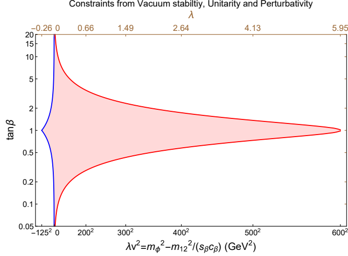
Figure 5. The shaded region indicates the surviving region of 2HDM parameter space of \tan \beta vs. \lambda v^2 , after vacuum stability (blue lines), unitarity and perturbativity (red lines) are taken into account. The corresponding values of \lambda are shown in the upper axis. Here we took the simplification of m_{H^\pm} = m_H = m_A \equiv m_\phi and alignment limit of \cos(\beta - \alpha) = 0 .
