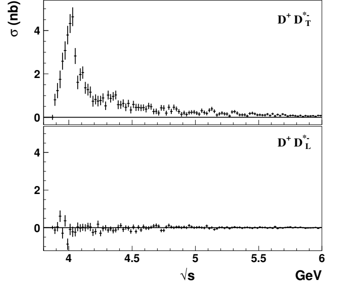
Fig. 18: The components of the e^+e^- \rightarrow D^+D^{*-}\gamma_{\text{ISR}} cross section corresponding to the different D^{*-} helicity: top is transverse; bottom is longitudinal.
