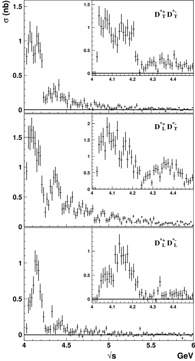
Fig. 21: The components of the e^+e^- \rightarrow D^{*\pm}D^{*-}\gamma_{\text{ISR}} cross section corresponding to the different D^{*\pm} 's helicities.
