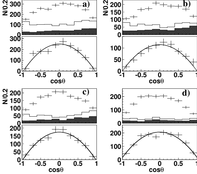
Fig. 17: The distribution of \cos\theta before (top panels) and after (bottom panels) background subtraction for different mass range: a) M(D^+D^{*-}) < 4.05 \text{ GeV}/c^2 , b) 4.05 \text{ GeV}/c^2 < M(D^+D^{*-}) < 4.3 \text{ GeV}/c^2 , c) 4.3 \text{ GeV}/c^2 < M(D^+D^{*-}) < 4.8 \text{ GeV}/c^2 , d) M(D^+D^{*-}) > 4.8 \text{ GeV}/c^2 . The contribution from the combinatorial background only is shown as the hatched histogram. The total contribution from the backgrounds sources is shown as the open histogram.
