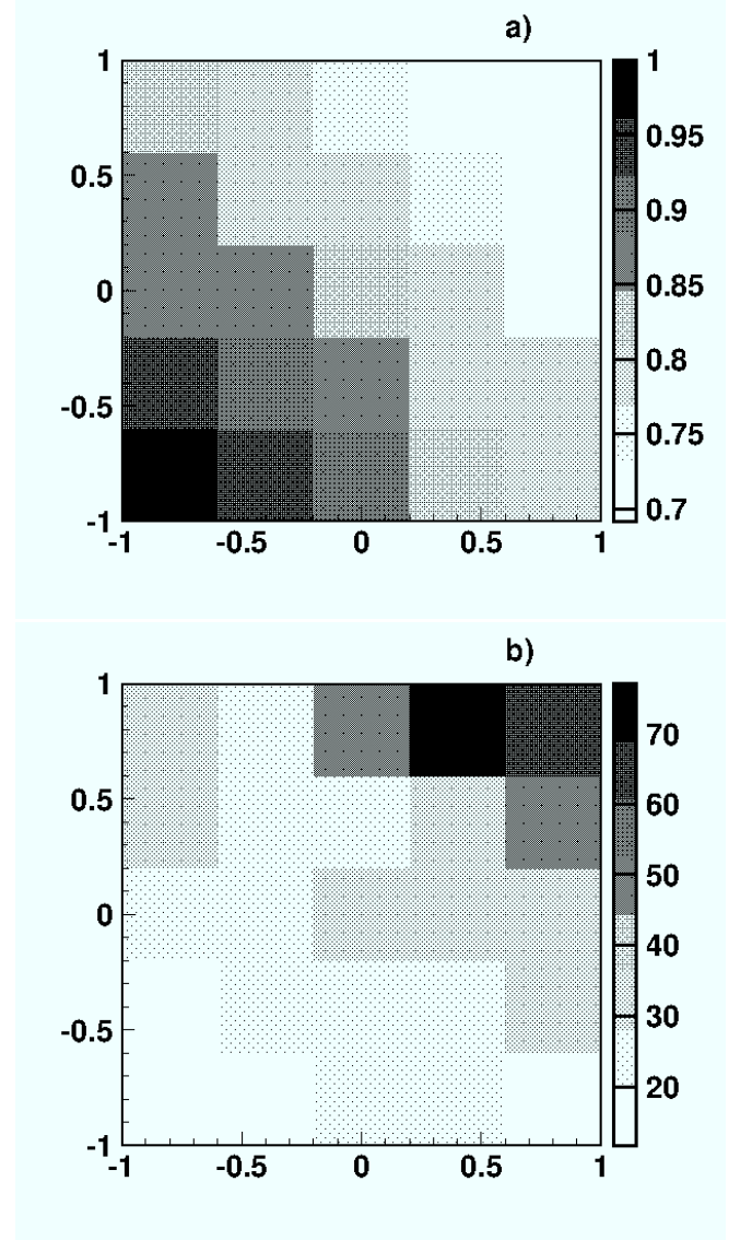
Fig. 20: The e^+e^- \rightarrow D^{*+}D^{*-}\gamma_{ISR} process: a) reconstruction efficiency as a function c_1 and c_2 ; b) total combinatorial background distribution.
