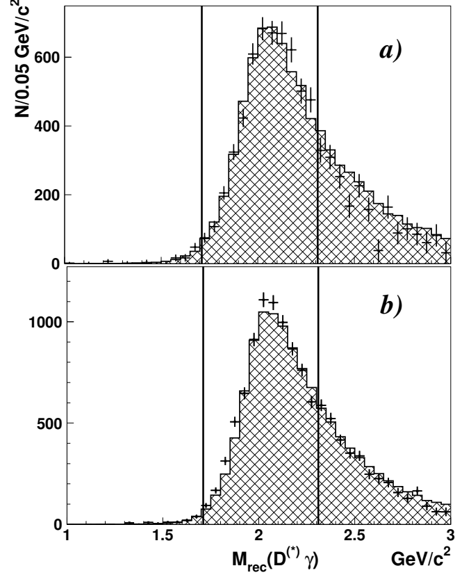
Fig. 14: a) The M_{\text{rec}}(D^+ \gamma_{\text{ISR}}) spectrum after subtraction of the combinatorial background and the contribution from the process e^+e^- \rightarrow D^{*+} D^{*-} \gamma_{\text{ISR}} for e^+e^- \rightarrow D^+ D^{*-} \gamma_{\text{ISR}} . b) The M_{\text{rec}}(D^{*+} \gamma_{\text{ISR}}) spectrum after combinatorial-background subtraction for e^+e^- \rightarrow D^{*+} D^{*-} \gamma_{\text{ISR}} . Points with error bars show the data after \gamma_{\text{ISR}} energy correction; the hatched histogram corresponds to the MC simulation. The signal window lies between the vertical lines.
