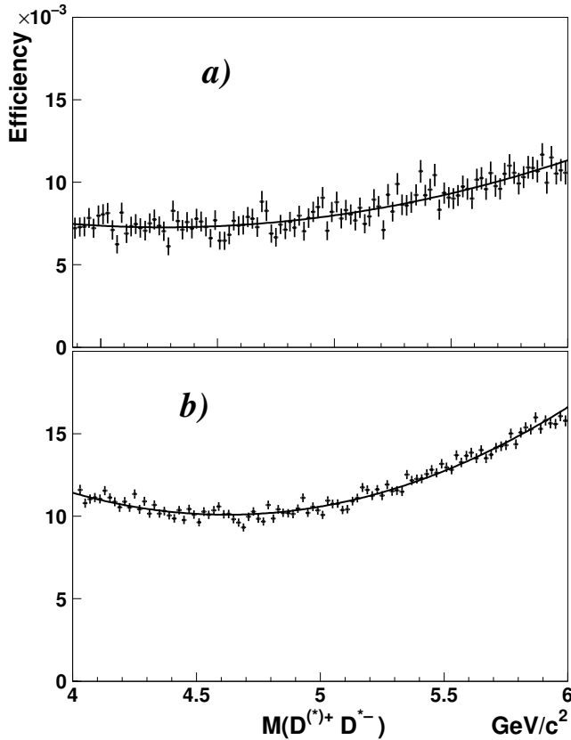
Fig. 15: The total efficiency as a function of M(D^{(*)+} D^{*-}) for a) e^+e^- \rightarrow D^+ D^{*-} \gamma_{ISR} and b) e^+e^- \rightarrow D^{*+} D^{*-} \gamma_{ISR} .
