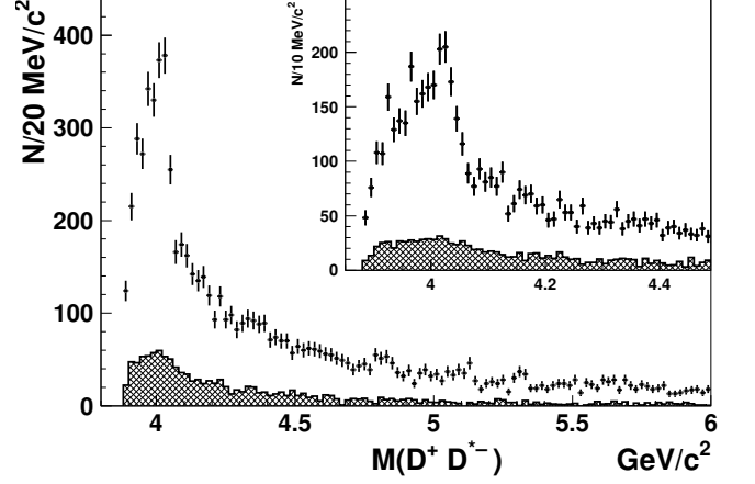
Fig. 9: The M(D^+D^{*-}) spectrum in the data after applying all selection criteria (points with error bars). The sum of backgrounds (1)-(3) is shown as the hatched histogram. The inset shows the spectrum near the threshold with finer bins
