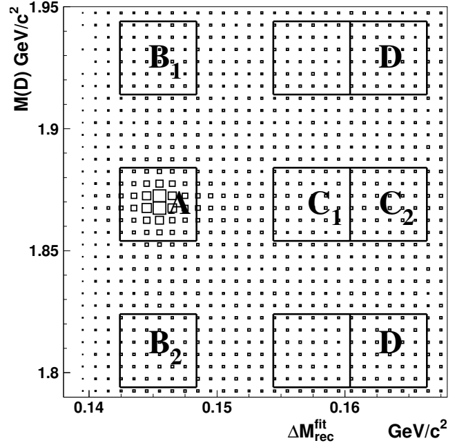
Fig. 10: The M(D^+) vs. \Delta M^{\text{fit}}_{\text{rec}} scatter plot in the data.
