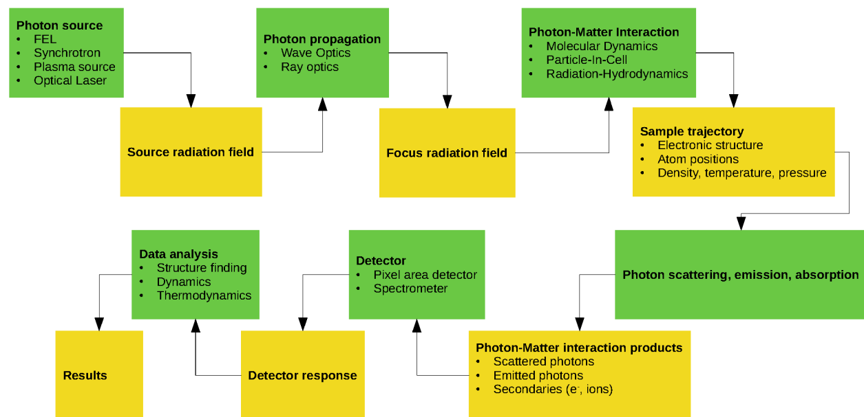
Fig 1 Baseline workflow in simex_platform . Green boxes represent Calculators , yellow boxes are data interfaces.
