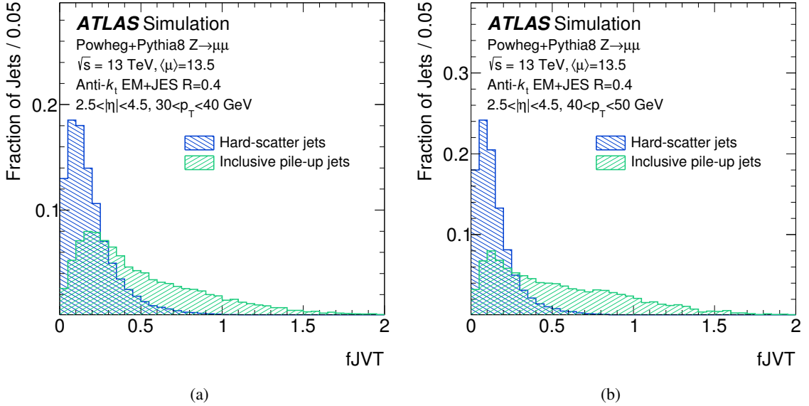
Figure 13: The fJVT distribution for hard-scatter (blue) and pile-up (green) forward jets in simulated Z+jet events with at least one forward jet with (a) 30 < p_T < 40 GeV or (b) 40 < p_T < 50 GeV.
