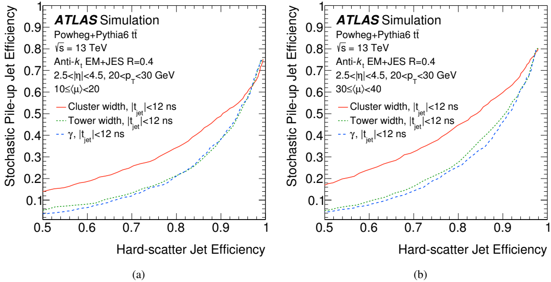
Figure 9: Efficiency for stochastic pile-up jets as a function of the efficiency for hard-scatter jets using different shape-based discriminants: (a) 10 \leq \langle \mu \rangle < 20 and (b) 30 \leq \langle \mu \rangle < 40 in simulated t\bar{t} events.
