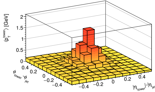
Figure 7: Distribution of the average tower p_T for hard-scatter jets as a function of the angular distance from the jet axis in \eta and \phi in simulated t\bar{t} events.
