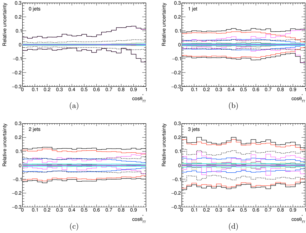
Figure A.30: Relative systematic uncertainties as a function of the cosine of the polar angle in the Collins-Soper frame for all inclusive jet categories.
