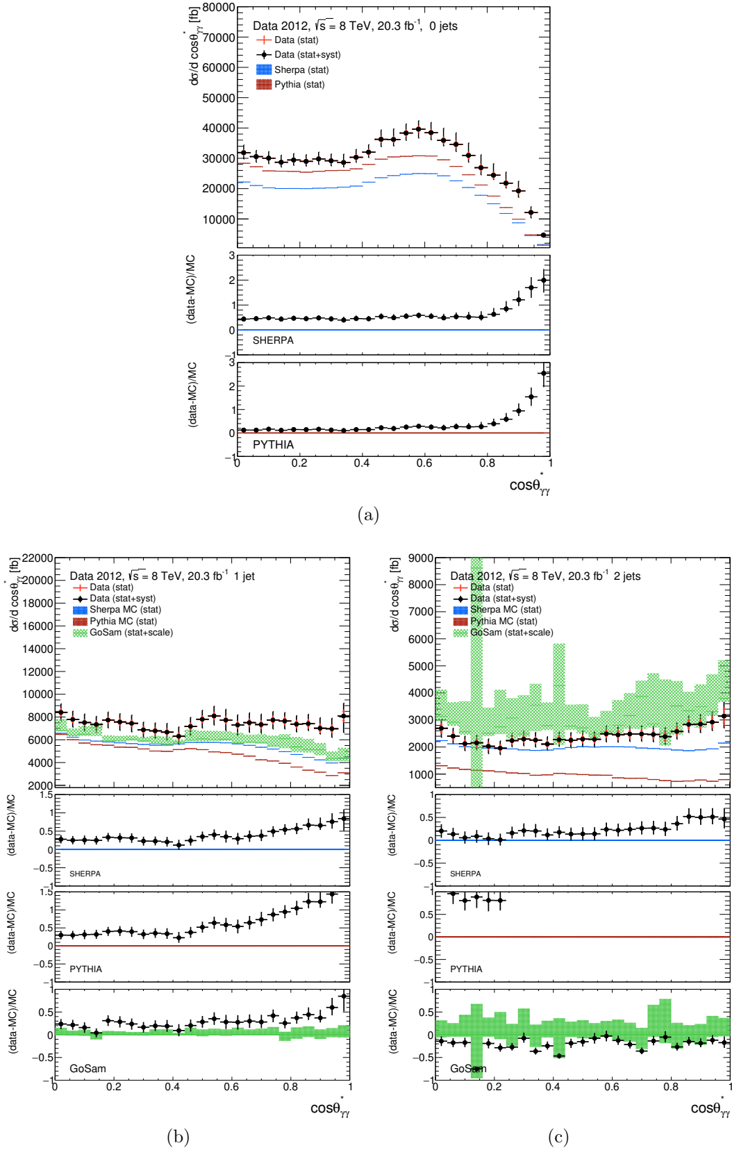
Figure A.3: Cross sections as a function of the cosine of the polar angle in the Collins-Soper frame for the 0-jet, 1-jet and 2-jet categories.
