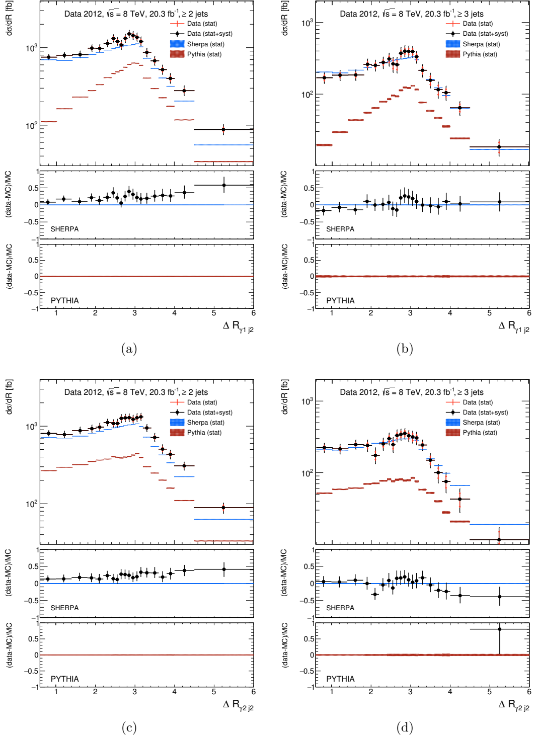
Figure A.17: Cross sections as a function of the distance between leading photon and subleading jet (a,b) and between subleading photon and subleading jet (c,d) for all inclusive jet categories.
