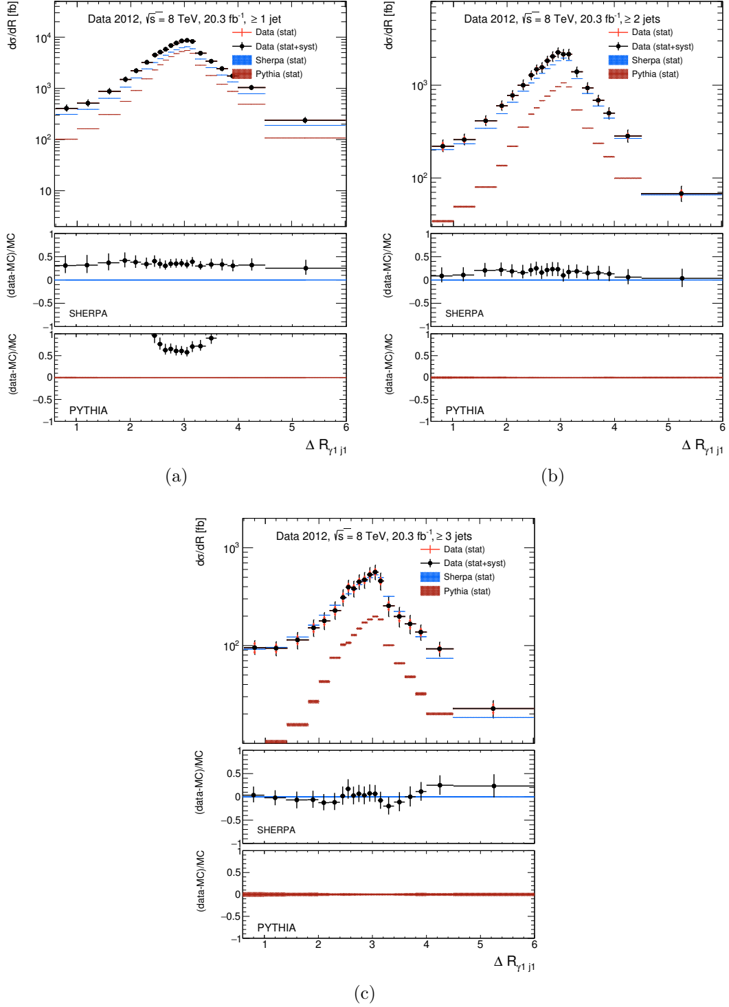
Figure A.15: Cross sections as a function of the distance between leading photon and leading jet for all inclusive jet categories.
