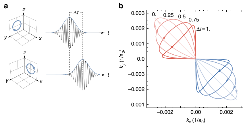
Figure 3 | Dynamical Floquet-Weyl points. (a) Floquet TDDFT predicts that the position of the Floquet-Weyl points can be controlled in real time on the timescale of pulse envelopes, yielding a time-dependent band structure that is accessible through time- and angle-resolved photoemission spectroscopy. Two time-delayed ( \Delta t ) pump laser pulses, circularly polarized in y - z and x - z directions, respectively, drive the Floquet-Weyl points in the k_x - k_y plane of the BZ. (b) The varying field strength during the laser pulses leads to dancing Floquet-Weyl points with trajectories controlled by \Delta t given in units of the FWHM of pulse envelopes.
