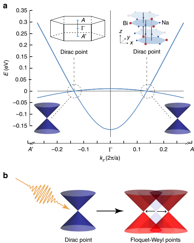
Figure 1 | Laser-induced Floquet-Weyl semimetal. (a) With intact time-reversal symmetry, doubly degenerate 3D Dirac cones exist at two Dirac points in \text{Na}_3\text{Bi} . Shown are the Dirac bands along a section of the A' - \Gamma - A path through the Brillouin zone, see left inset. The right inset shows the crystal structure of \text{Na}_3\text{Bi} . (b) Breaking time-reversal symmetry with circularly polarized light splits each Dirac cone into a pair of Floquet-Weyl cones.
