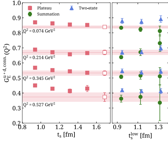
FIG. 8. Connected contribution to the G_E^{u+d}(Q^2) form factor, for four nonzero Q^2 values, extracted from the plateau method (squares), the summation method (filled circles) and the two-state fit method (filled triangles). The notation is the same as in Fig. 4.
