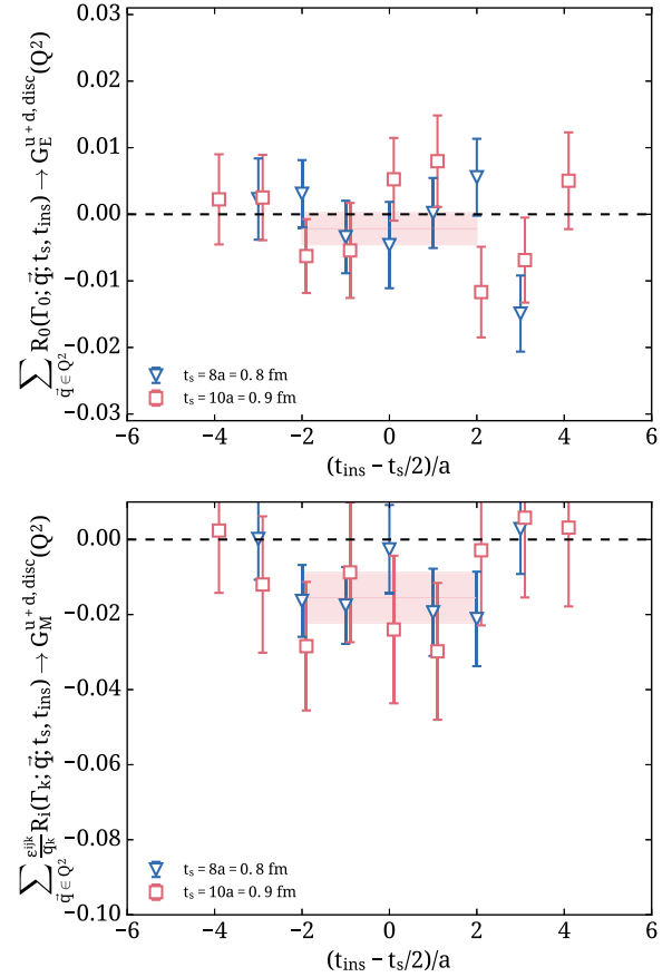
FIG. 10. Disconnected contribution to the electric (upper panel) and magnetic (lower panel) isoscalar Sachs form factors for sink-source separation t_s = 8a = 0.75 \text{ fm} (inverted triangles) and t_s = 10a = 0.94 \text{ fm} (squares) for the first nonzero momentum transfer of Q^2 = 0.074 \text{ GeV}^2 . The horizontal bands show the values obtained after fitting with the plateau method to the results at t_s = 10a = 0.94 \text{ fm} .
