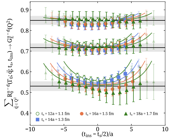
FIG. 2. Ratio yielding the isovector electric Sachs form factor. We show results for three representative Q^2 values, namely the first, second and fourth nonzero Q^2 values, for t_s = 12a (open circles), t_s = 14a (filled squares), t_s = 16a (filled circles) and t_s = 18a (filled triangles). The curves are the results from the two-state fits, with the fainter points excluded from the fit. The band is the form factor value extracted using the two-state fit.
