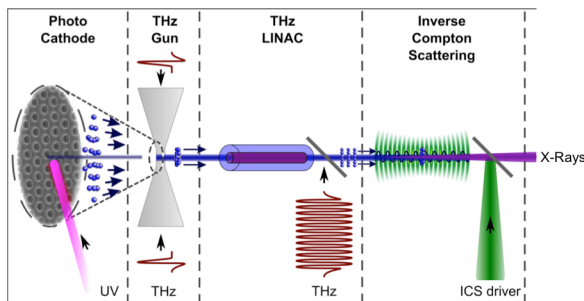
Fig. 1. Schematic of the AXSIS x-ray source
