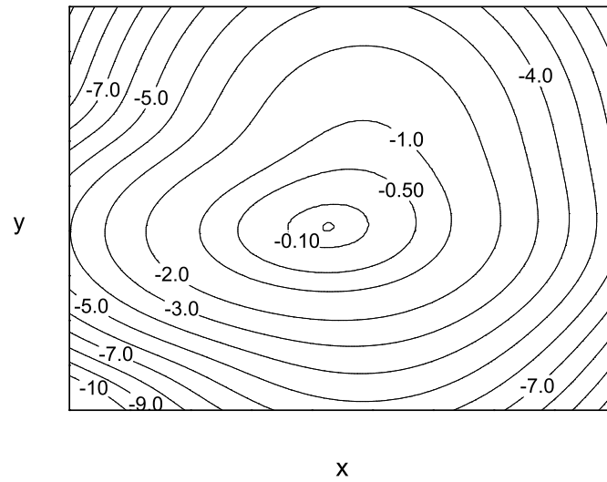
Fig. 6.8. Likelihood contours.
