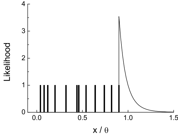
Fig. 6.13. Likelihood function of the width of a uniform distribution for 12 observations.
