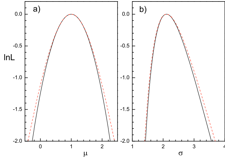
Fig. 6.6. Log-likelihood functions for the parameters of a normal distribution: a) for the mean \mu with know width (solid curve) and unknown width (dashed curve), b) for the width \sigma with known mean (solid curve) and unknown mean (dashed curve). The curves represent expected likelihoods for 10 events.
