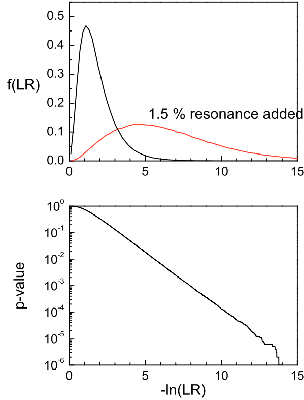
Fig. 10.20. Distributions of the test statistic for H_0 and for experiments with a 1.5% resonance contribution. In the lower graph the p -value for H_0 is given as a function of the test statistic.
