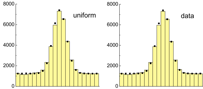
Fig. 9.11. Iterative unfolding with two different starting histograms, left uniform and right experimental.
