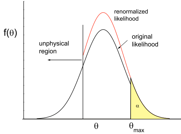
Fig. 8.6. Renormalized likelihood function and upper limit.
