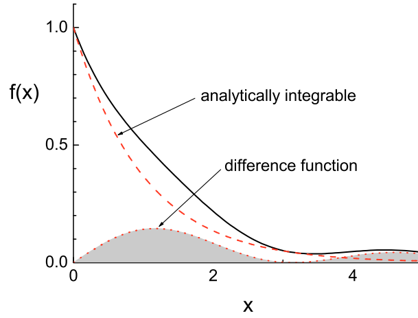
Fig. 5.13. Monte Carlo integration of the difference between the function to be integrated and an integrable function.
