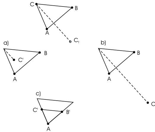
Fig. 13.6. Simplex algorithm.
