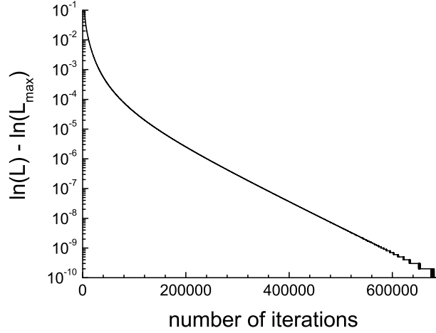
Fig. 9.18. Difference of the log-likelihood from the value at 10^6 iterations as a function of the number of iterations.
