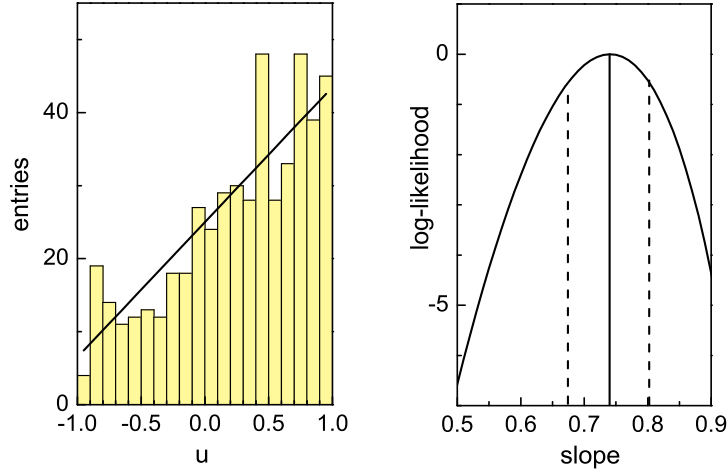
Fig. 7.1. Linear distribution with adjusted straight line (left) and likelihood function (right).
