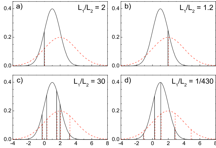
Fig. 6.4. Likelihood ratio for two normal distributions. Top: 1 observation, bottom: 5 observations.
