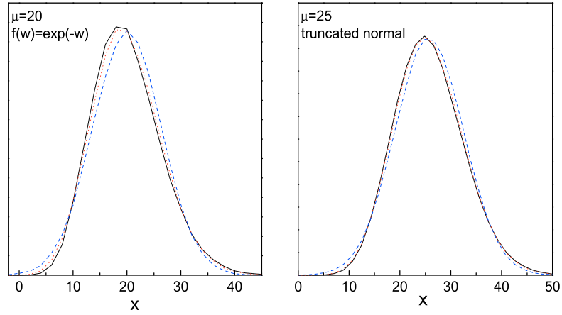
Fig. 13.5. comparison of a CPD with a scaled Poisson distribution(doted) and a normal approximation (dashed).
