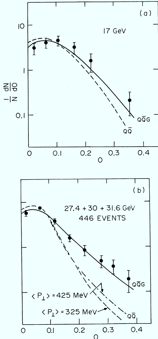
FIG. 2. (a) The distribution N^{-1}dN/dO as function of oblateness at \sqrt{s} = 17 GeV. (b) The distribution N^{-1}dN/dO as function of oblateness at \sqrt{s} = 27.4 - 31.6 GeV. In both (a) and (b) the solid curves are the predictions based on the q\bar{q}g model and the dashed curve is based on the standard q\bar{q} model with \langle P_{\perp} \rangle = 325 MeV. The dash-dotted curve in (b) is the q\bar{q} model prediction with \langle P_{\perp} \rangle = 425 MeV.
