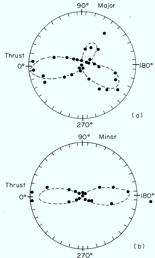
FIG. 3. (a) Energy distribution in the plane as defined by the thrust and the major axes for all the events with thrust < 0.8 and oblateness > 0.1 at \sqrt{s} = 27.4, 30 , and 31.6 GeV. The energy value is proportional to the radial distances. The superimposed dashed line represents the distribution calculated with use of the q\bar{q}g model. (b) The measured and calculated energy distribution in the plane as defined by the thrust and the minor axes.
