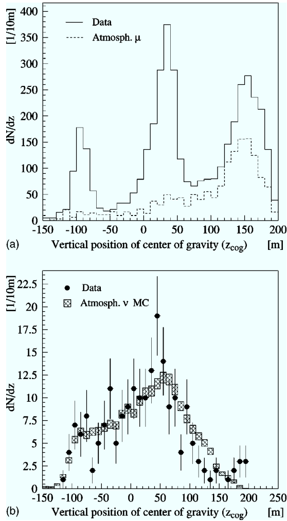
FIG. 14. Top: Event center of gravity distribution after reconstruction with special cross-talk cleaning algorithms applied to the events. Unsimulated background remains. Bottom: The data agree with the neutrino signal after application of additional quality cuts.
