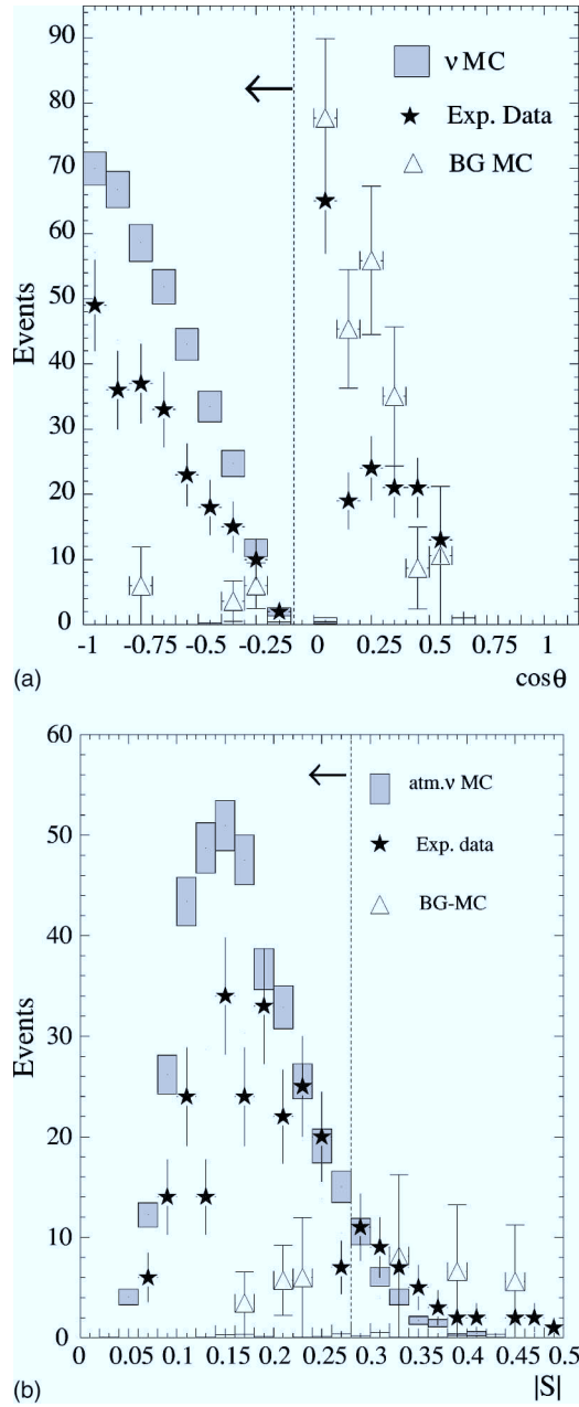
FIG. 11. Two distributions of variables used as cut parameters in the last filter level (see Table I for an explanation of the variables). In both cases, all final cuts with the exception of the variable plotted have been applied. The cuts on the displayed parameters are indicated by the dashed vertical lines. Arrows indicate the accepted parameter space.
