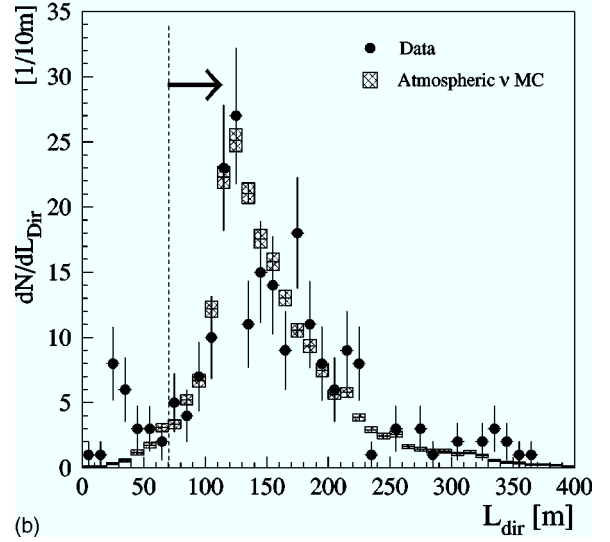
FIG. 19. Smoothness and direct length variables where quality level 7 cuts have been applied in all but the displayed variable ( N - 1 cuts; see also Sec. V D 3, Fig. 11). The vertical dashed lines with the arrow indicate the region of acceptance in the displayed variable. In each case, a clear tail of fake events is removed by application of the cut, leaving good agreement in shape between the remaining events and the Monte Carlo expectation.
