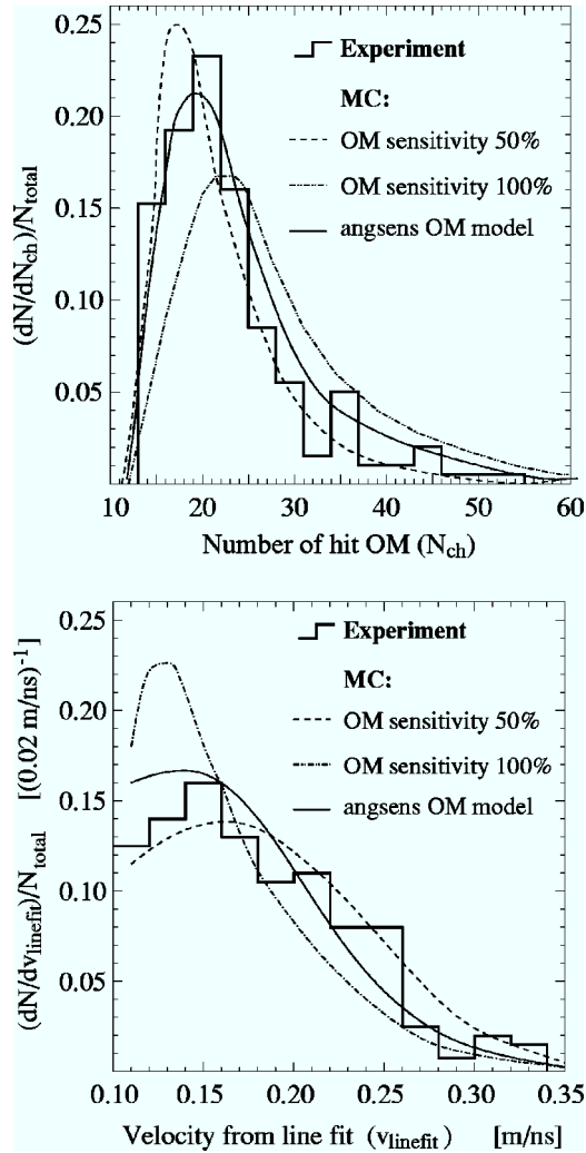
FIG. 20. Distributions of two variables that are affected by the OM sensitivity, comparing different signal Monte Carlos events to the observed data. Top: the number of OMs hit ( N_{ch} ); bottom: the event velocity for a simplified fit (line fit, v_{linefit} ).
