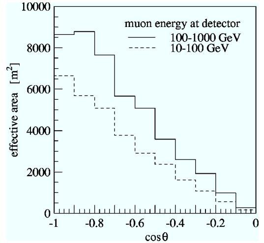
FIG. 23. Effective area for muons versus zenith angle. The energy of the muons is given at the point of closest approach to the detector.
