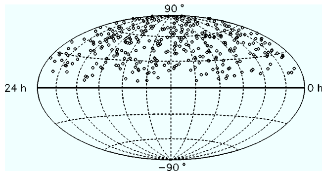
FIG. 25. Neutrino skyplot of upgoing events as seen with AMANDA-B10 in 1997 in equatorial coordinates. In this figure, neutrino events from both analyses are combined. The background of non-neutrino events is estimated to be less than 10%.
