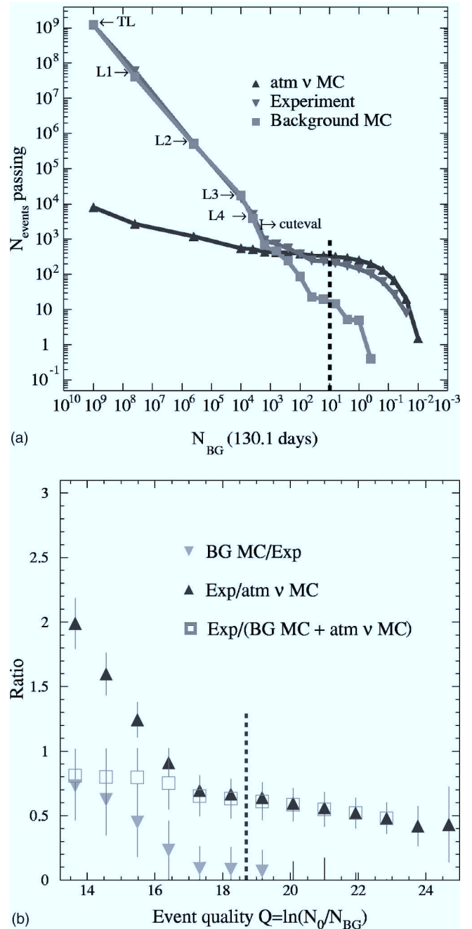
FIG. 8. The fitted background parameter N_{\text{BG}} . Top: Number of events versus N_{\text{BG}} . Smaller values of N_{\text{BG}} correspond to harder cuts. Below N_{\text{BG}} = 1500 the CUTEVAL parametrization was used to calculate the cut values corresponding to N_{\text{BG}} . For larger values of N_{\text{BG}} the data points correspond to the cuts from the filter levels: Level 4 (see Sec. V B), level 3, level 2, level 1, and trigger level (Table II). Bottom: Ratios of events passing in the experimental data compared to various Monte Carlo expectations for signal and background as a function of event quality. The dashed line indicates the final cuts.
