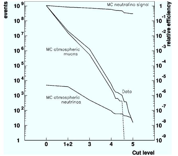
FIG. 2. Rejection and efficiency at each filter level for the data and simulations of the neutralino signal, atmospheric neutrinos and atmospheric muons. The dashed part corresponds to rejection levels surpassing the statistical precision of the simulated sample, yielding zero remaining events. The neutralino signal curve should be read only with respect to the right axis scale, and it shows the relative signal efficiency with respect to trigger level. The rest of the curves are plotted with respect to the left axis scale.
