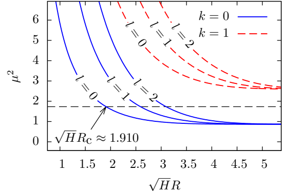
Figure 3: The lowest eigenvalues corresponding to positive color orientation \kappa^a = 1 as functions of \sqrt{HR} . The critical radius R_c corresponds to \mu_{a00}^2 = 2v = \sqrt{3} . For large \sqrt{HR} eigenvalues approach correct Landau levels, the degeneracy in l is restored.
