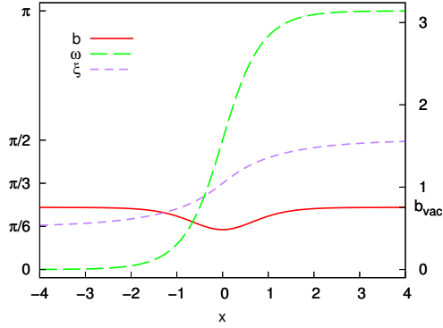
Figure 1: Kink connecting distinct vacua. Angle \omega varies from 0 to \pi , angle \xi varies from \pi/6 to \pi/2 . Global minima of effective potential (1) are degenerate in the value of field strength b = b_{\text{vac}} , so its magnitude is the same for all vacua. Dimensionless variable x \equiv \Lambda x is used.
