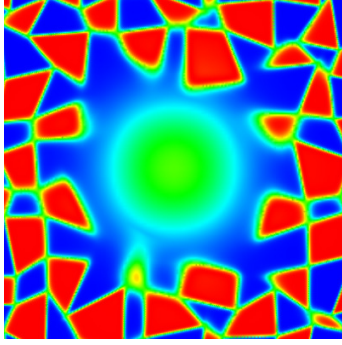
Figure 2: Example of two-dimensional slice of the cylindrical thick domain wall junction. Self-dual and anti-self-dual fields are indicated by blue and red colors respectively. The topological charge density vanishes inside the junction (green color).
