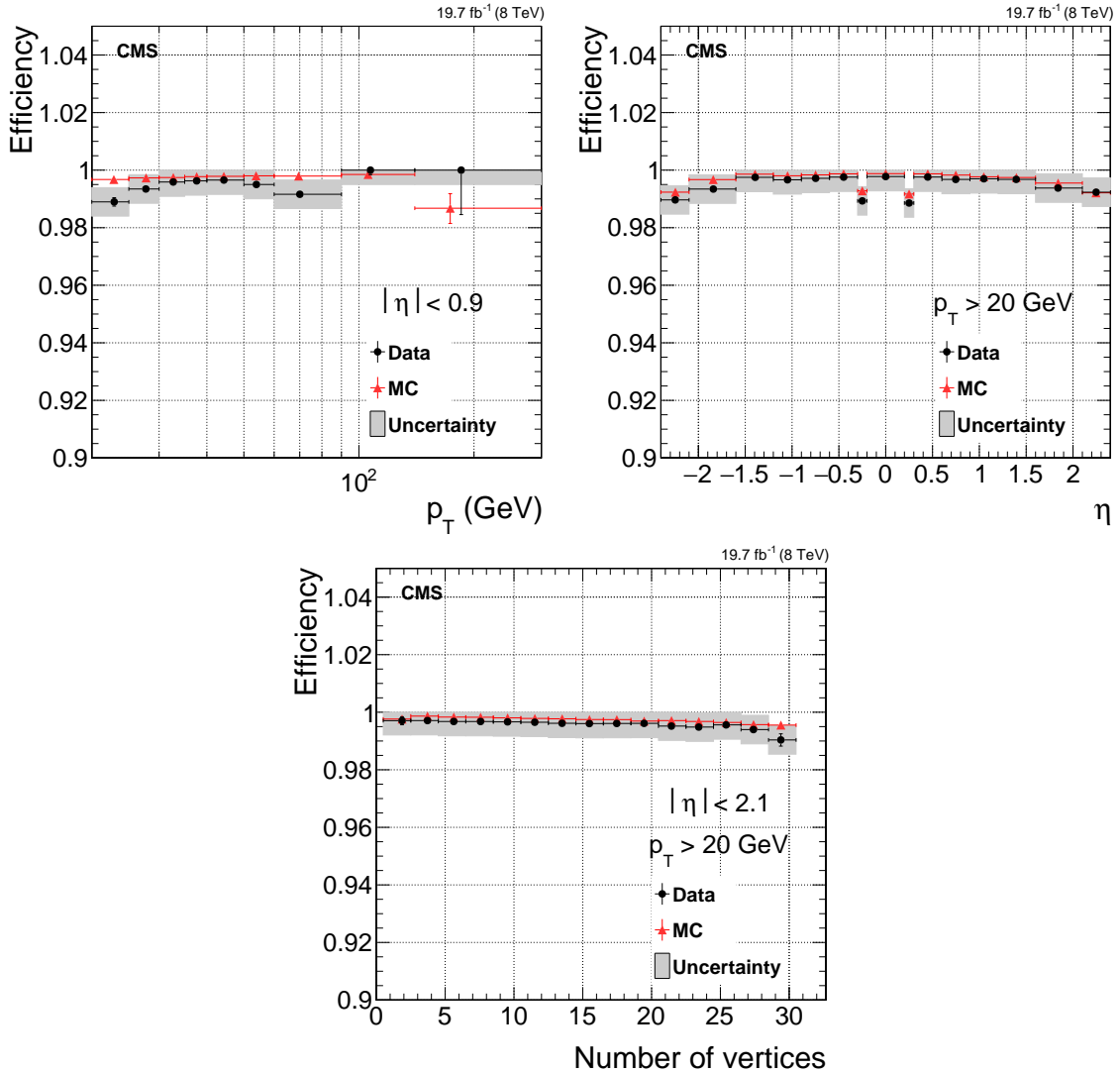
Figure 29: Efficiency of the PF muon identification for muons from Z boson decays as a function of p_T (top left), \eta (top right), and N_{\text{vtx}} (bottom).
