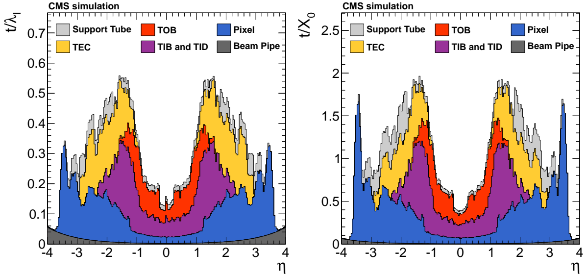
Figure 3: Total thickness t of the inner tracker material expressed in units of interaction lengths \lambda_1 (left) and radiation lengths X_0 (right), as a function of the pseudorapidity \eta . The acronyms TIB, TID, TOB, and TEC stand for “tracker inner barrel”, “tracker inner disks”, “tracker outer barrel”, and “tracker endcaps”, respectively. The two figures are taken from Ref. [18].
