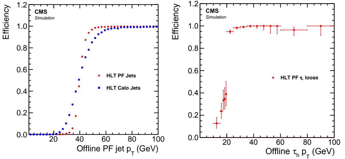
Figure 22: Left: Probability to find at HLT a jet with p_T > 40 GeV matching the jet reconstructed offline, as a function of the offline jet p_T . At the threshold, the curve is steeper for HLT PF jets (circles) than for HLT calorimeter jets (squares). Right: Probability to find a \tau_h with p_T > 20 GeV at HLT matching the \tau_h reconstructed and identified offline with the loose isolation working point.
