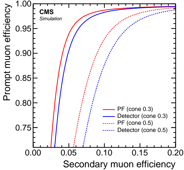
Figure 18: Isolation efficiency for muons from W boson decays versus isolation efficiency for muons from secondary decays, both obtained from simulated t\bar{t} events, as a function of the threshold on the isolation for the detector- and particle-based methods. The efficiencies are shown for two choices of the maximum \Delta R (isolation cone size): 0.3 and 0.5.
