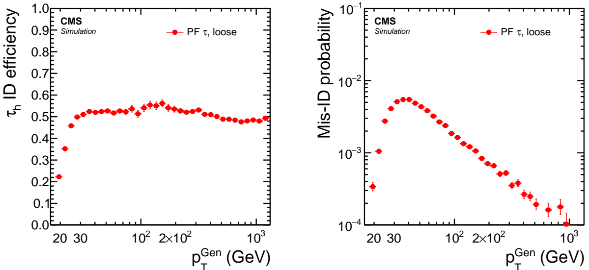
Figure 21: Identification efficiency for genuine \tau_h (left), and \tau_h misidentification probability for quark and gluon jets (right). Low- p_T \tau_h are obtained from simulated Z/\gamma^* \rightarrow \tau\tau events and high- p_T \tau_h from simulated H(3.2 \text{ TeV}) \rightarrow \tau\tau events. Quark and gluon jets are obtained from simulated QCD multijet events. The \tau_h are required to be reconstructed by the HPS (PF) algorithm, to have p_T > 20 \text{ GeV} and |\eta| < 2.3 , and to satisfy the loose \tau_h identification criteria.
