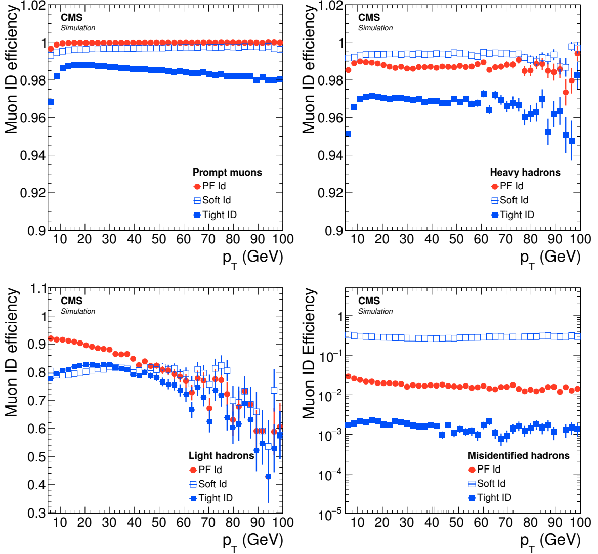
Figure 17: Efficiency for different algorithms (PF, soft, and tight) to identify a simulated muon track that has been reconstructed as a tracker muon, as a function of the p_T of the reconstructed track. From top left to bottom right the efficiency of the three identification algorithms is shown for prompt muons, for muons from heavy-flavour decays, for muons from light-flavour decays, and for misidentified hadrons.
