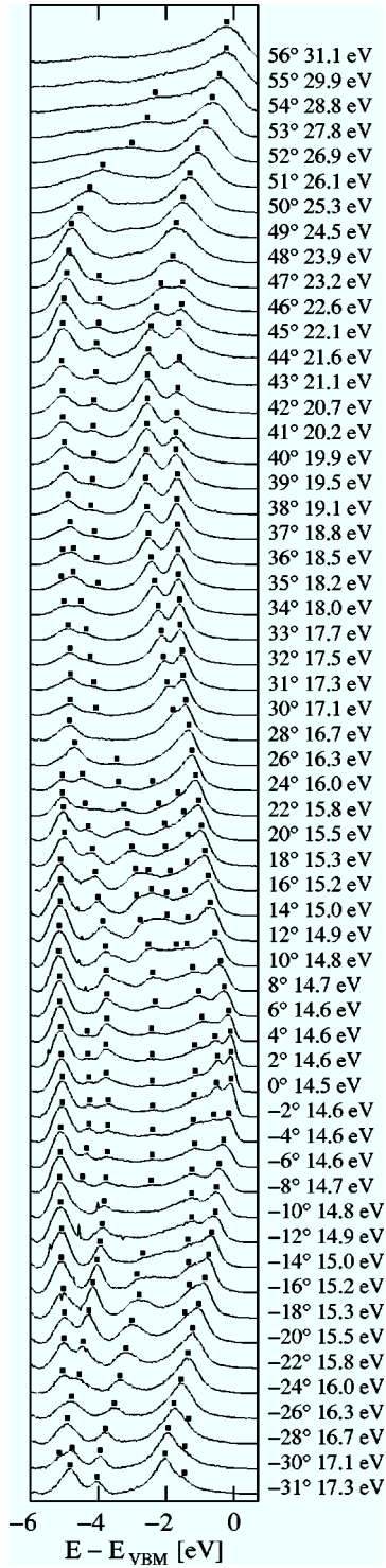
FIG. 6. Off-normal emission spectra in the \Gamma KWX plane from ZnSe(001). Dispersive spectral features are indicated by bars.
