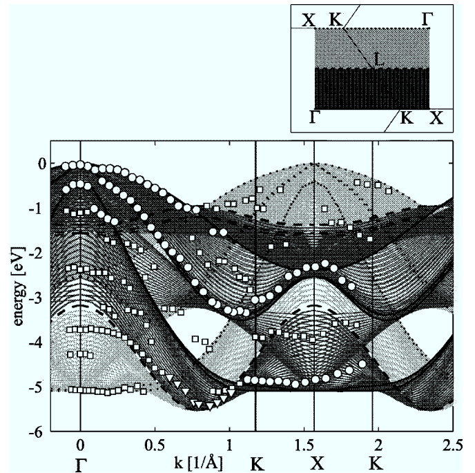
FIG. 9. The band structure for \Gamma KLUX plane constructed assuming free-electron final states. Circles show bulk-related primary-cone features. Squares and triangles indicate other dispersions that cannot be explained as primary-cone free-electron features. Darker gray areas show the projected bulk band structure for \Gamma KLUX plane for k_{\perp} from 0 to \pi/a and lighter gray areas for k_{\perp} from \pi/a to 2\pi/a . Solid lines show bands in \Gamma KLUX plane at k_{\perp}=0 (along \Gamma -K-X), dashed lines for k_{\perp}=\pi/a (this includes L point), and dotted lines for k_{\perp}=2\pi/a (along X-K- \Gamma ). It is also schematically shown on the top-right of the figure in the BZ section. See the text for details.
