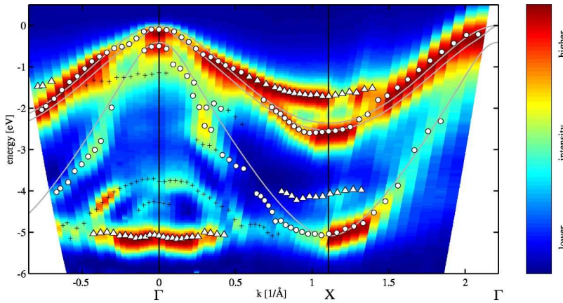
FIG. 7. (Color online) Band structure constructed using the features indicated in Fig. 6. Circles indicate primary-cone bulk related features, triangles indicate surface related features and the nondispersive feature at around -5 eV, and crosses indicate secondary-cone emissions or features related to final-state effects. Solid lines show the theoretical band structure along \Gamma -X. Color map areas represent the same spectra as in Fig. 6 but plotted in the E(k) plane with k vectors calculated using Eq. (3).
