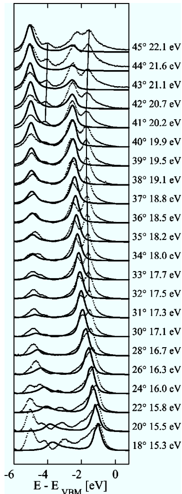
FIG. 8. Comparison of the experimental (dots) and theoretical (solid lines) spectra for off-normal emission in the \Gamma KWX plane. Surface related features are indicated by the guidelines. The experimental spectra are a selection from Fig. 6.
