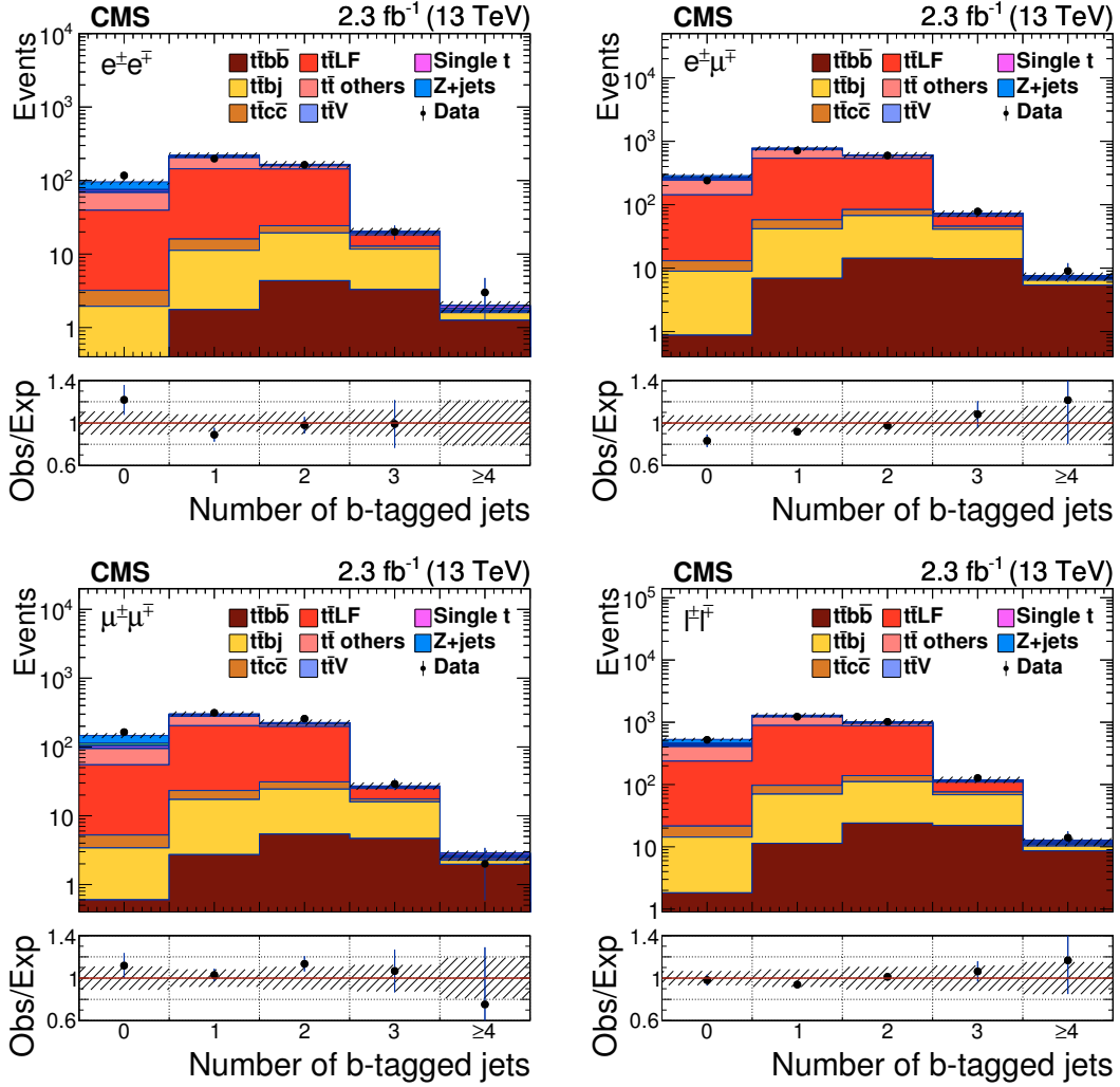
Figure 3: Distribution of b jet multiplicity after the four-jet requirement, but without the b tagging requirement, for the e^+e^- (upper left), e^+\mu^- (upper right), and \mu^+\mu^- (lower left) final states and the sum of the three final states (lower right). The points show the data and the stacked histograms are from simulated events, normalized by the results of the fit. The ratio of the number of data events to the expected number, as given by the stacked histograms, is shown in the lower panels. The hatched region indicates the modelling uncertainty in the MC simulation.
