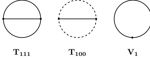
Figure 2: Two-loop and one-loop master integrals. The line coding is the same as in Fig. 1.
