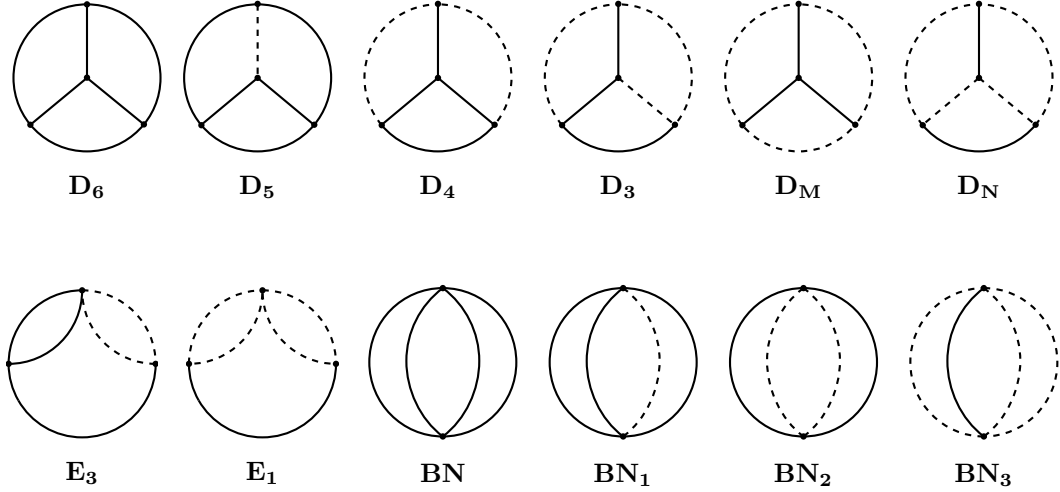
Figure 1: Full set of non-factorizing master integrals. Solid and dashed lines correspond to the massive and massless scalar propagators, respectively.
