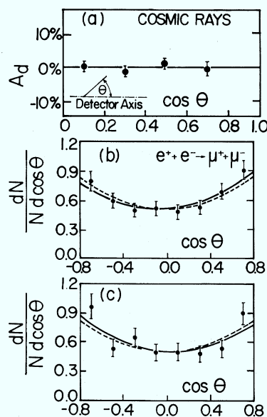
FIG. 1. (a) The measured detector asymmetry A_d defined as the percentage difference in acceptance for positive and negative muons as a function of the polar angle, as determined from 20 000 cosmic-ray events with momenta between 10 and 50 GeV/c. The angular distribution of muon-pair events as a function of the cosine of the scattering angle, for (b) \sqrt{s}=14 GeV and (c) \sqrt{s}=22 GeV, corrected for detector acceptance and the \alpha^3 QED angular asymmetry. The full curves are fits to the data, under the assumption of Eq. (2). The dashed curves represent the angular distribution due to the lowest-order QED alone.
