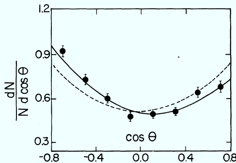
FIG. 2. Same as Figs. 1(b) and 1(c) at \sqrt{s}=34.6 GeV, showing the electroweak effect.
