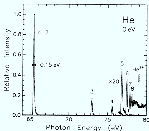
FIG. 3. Threshold photoelectron scan of the He satellites. n is the principal quantum number of the remaining electron in \text{He}^+ . The count rate at the maximum of the n=2 satellite peak is 9700 counts per second. The line simply connects the data points.
