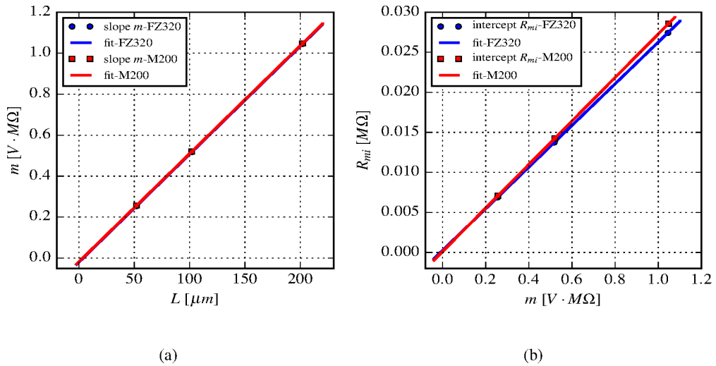
Figure 3.8: (a) Slope m as a function of L and (b) Intercept R_{mi} as a function of m for the FZ320 and M200 rectangular p-MOSFETs <100> .
