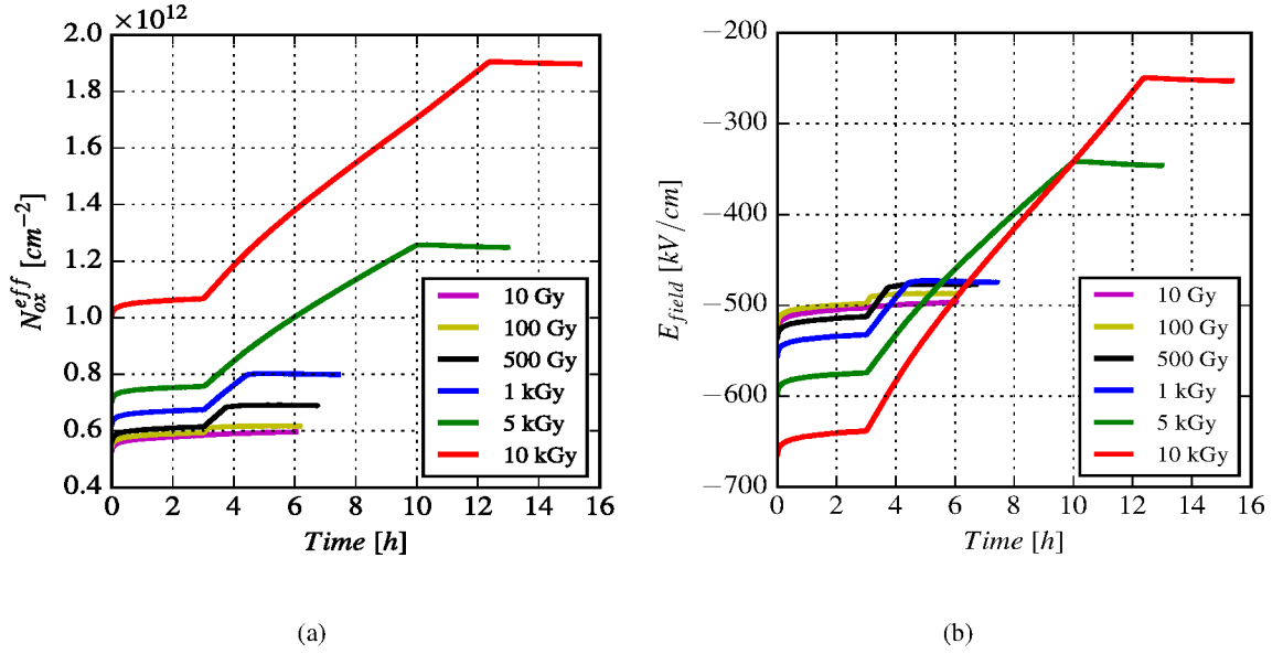
Figure 5.8: (a) Effective oxide charge density, N_{ox}^{eff}(t) and (b) Electric field E_{field} as a function of time for the individual irradiation cycles of p-MOSFET irradiated with E_{field} \uparrow .
