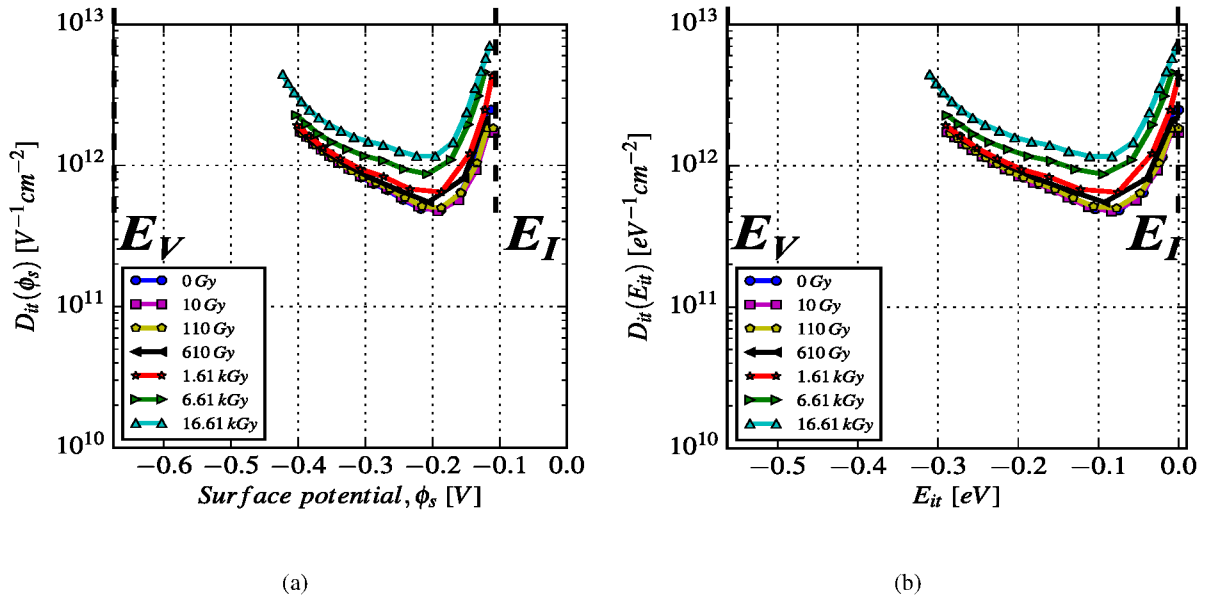
Figure 6.11: (a) D_{it} as a function of the surface potential and, (b) Energy in the Si bandgap before and after X-ray irradiation of the p-MOSFET <111> irradiated with E_{field} \uparrow .
