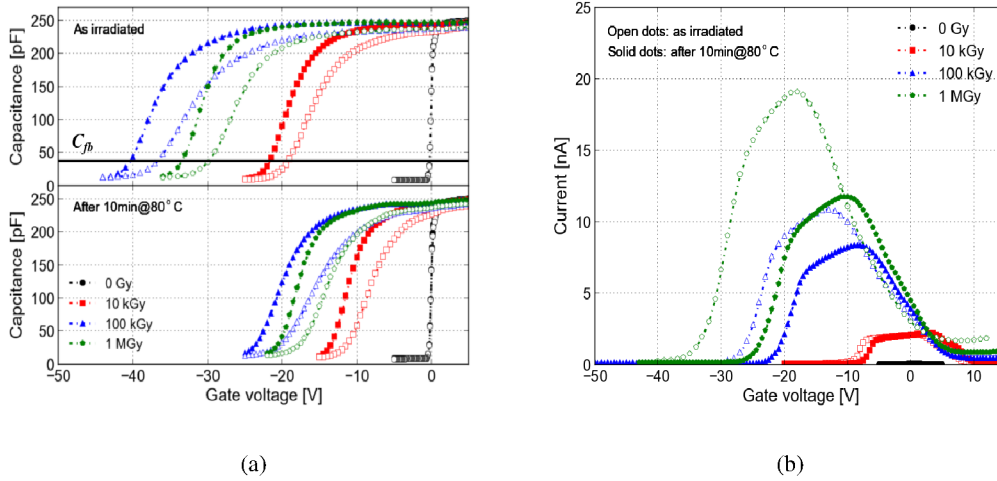
Figure 4.24: (a) C-V curves of the MOSC and (b) I-V curves of the GCD.
