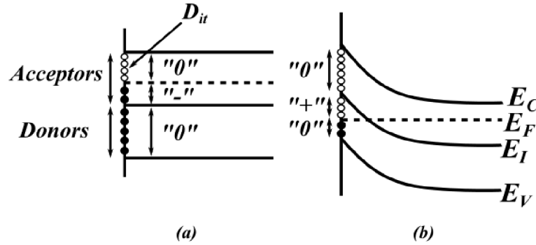
Figure 4.13: Band diagrams of p-MOSFET (n-type Si) showing the occupancy of interface traps with (a) negative interface trap charge at flatband and (b) positive interface trap charge at inversion. Figure adapted from [81].
