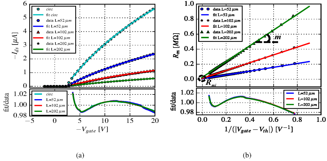
Figure 3.6: (a) I_{ds} as a function of V_{gate} and the parametrization fit used to determine the threshold voltage V_{th} and the hole mobility of the circular and rectangular p-MOSFETs <100> and (b) R_m as a function of 1/(|V_{gate} - V_{th}|) and the parametrization fit used to determine the slope m and the intercept R_{mi} of the rectangular p-MOSFETs <100>.
