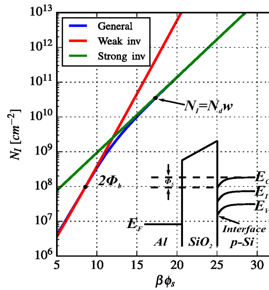
Figure 2.2: Inversion layer carrier density per unit area N_I as a function of band bending \phi_s . The red line is for weak inversion, the green line is for strong inversion, and the blue line is the general case.
