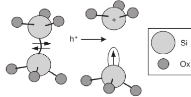
Figure 4.8: Model for hole trapping and E' center formation in SiO 2 . Figure taken from [81].
