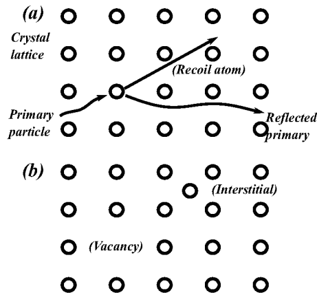
Figure 4.4: Atomic displacement damage in crystalline solid: (a) Atomic displacement event and (b) Simple radiation-induced defects (vacancy and interstitial). Atom displacements produce lattice defects which result in localized trap states-energy levels within bandgap. Figure adapted from [64].
