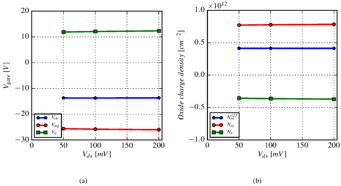
Figure 9.2: (a) Gate voltage and, (b) Oxide charge density for different V_{ds} values of the n-MOSFET <100> irradiated with E_{field} ↓ at 1.25 kGy X-ray dose.
