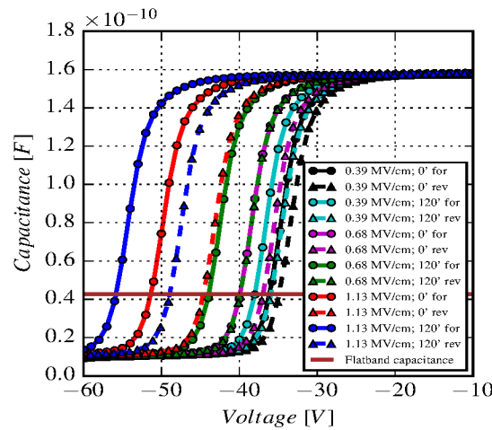
Figure 4.26: C-V curves at 10 kHz for the irradiated \langle 111 \rangle MOSC measured at -20 °C for the 3 values of V_{inv} and t_{bias} = 0 and 120 min. The results for the forward (f) and for the reverse (r) voltage ramping are shown. The horizontal line gives the value of the flatband capacitance. Data taken from [117].
