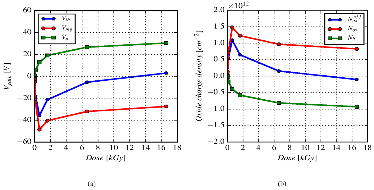
Figure 6.17: (a) Gate voltage and, (b) Oxide charge density as a function of X-ray dose of the n-MOSFET <100> irradiated with E_{field} \uparrow .
