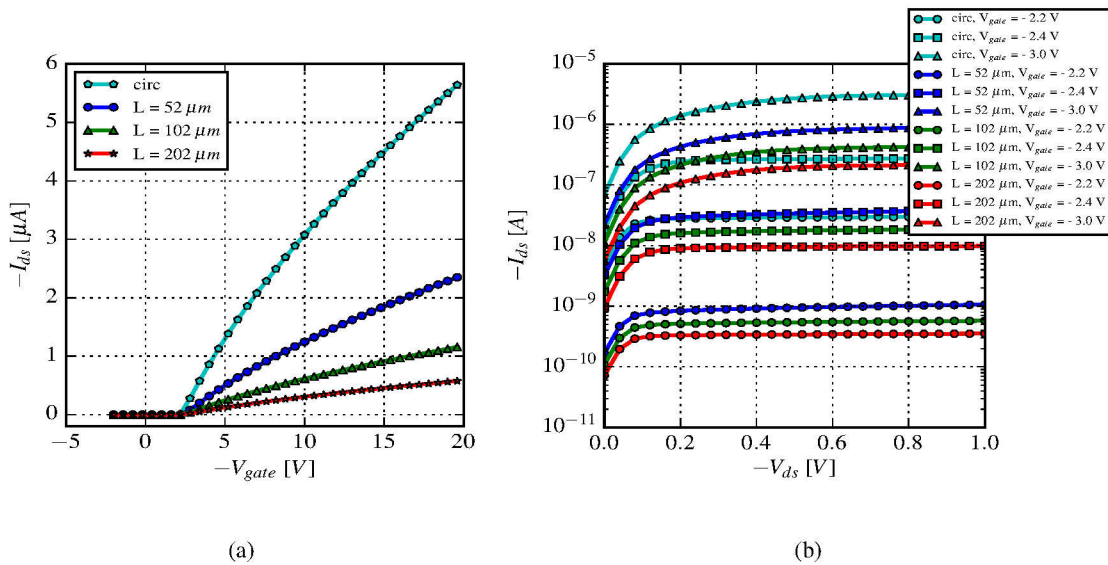
Figure 3.3: (a) I_{ds} as a function of V_{gate} in the linear region, V_{ds} = -50 mV, and (b) I_{ds} as a function of V_{ds} for three V_{gate} values of the circular and the three rectangular p-MOSFETs <100>.
