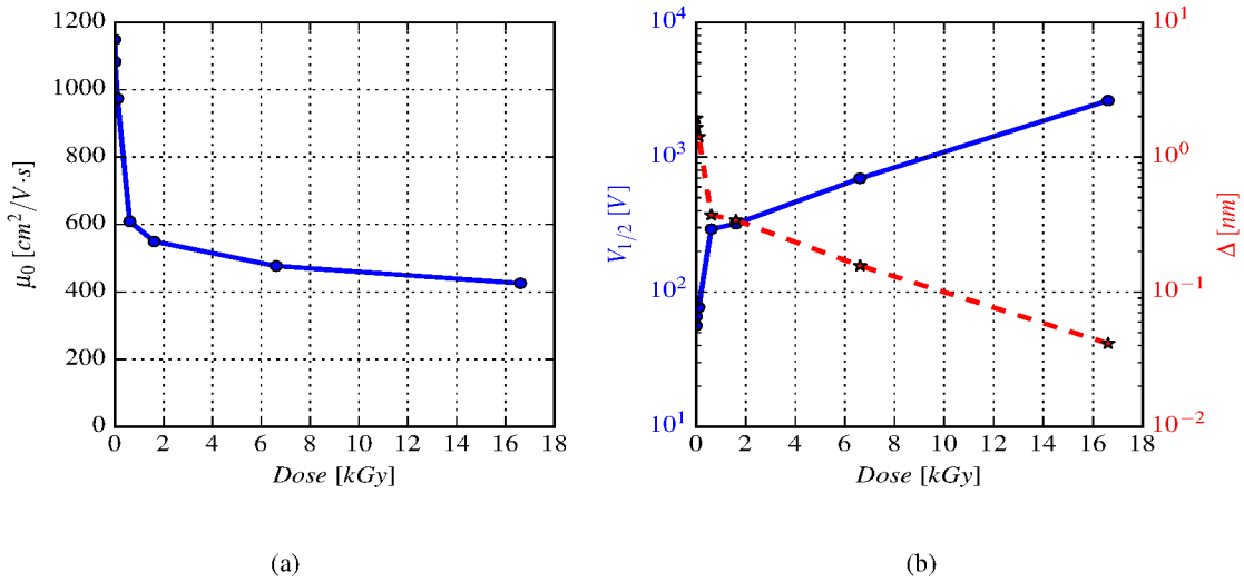
Figure 5.22: (a) Electron mobility, \mu_0 , and (b) V_{1/2} and \Delta as a function of the accumulated X-ray dose of n-MOSFET irradiated with E_{field} \uparrow .
