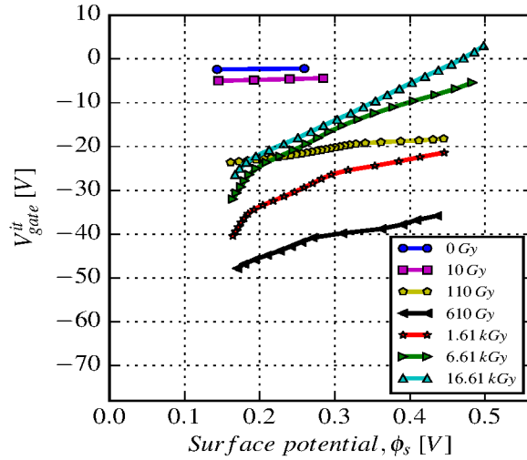
Figure 6.18: Gate voltage as a function of surface potential in the subthreshold region before and after X-ray irradiation of the n-MOSFET <100> irradiated with E_{field} \uparrow .
