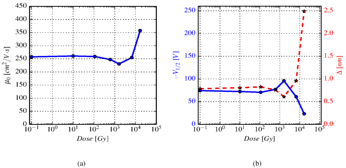
Figure 5.16: (a) Hole mobility, \mu_0 , and (b) V_{1/2} and \Delta as a function of the accumulated X-ray dose of p-MOSFET irradiated with E_{field} ↓.
