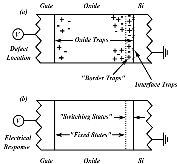
Figure 5.36: Diagram that illustrates a revised defect nomenclature for MOS devices which distinguishes terms used to describe (a) the physical location of defects (b) from their electrical response. Figures adapted from [132].
