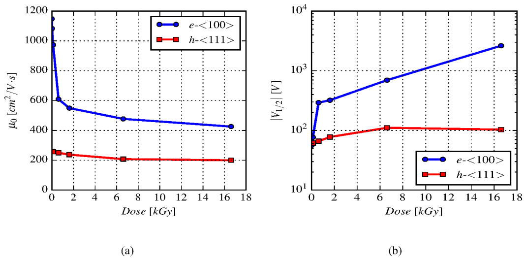
Figure 5.34: (a) Electron and hole mobility, \mu_0 , and (b) V_{1/2} as a function of the accumulated X-ray dose of n- and p-MOSFET irradiated with E_{field} \uparrow .
