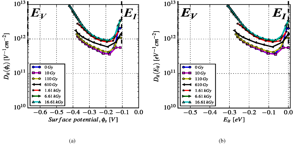
Figure 6.15: (a) D_{it} as a function of the surface potential and, (b) Energy in the Si bandgap before and after X-ray irradiation of the p-MOSFET <111> irradiated with E_{field} \downarrow .
