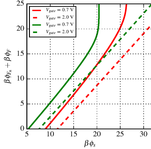
Figure 2.10: Electron quasi-Fermi level, \beta\phi_{F_n} as a function of \beta\phi_s for two V_{gate} values, green color for t_{ox} = 250 nm, N_d = 6.2 \cdot 10^{11} \text{ cm}^{-3} and red color for t_{ox} = 700 nm, N_d = 4.4 \cdot 10^{12} \text{ cm}^{-3} .
