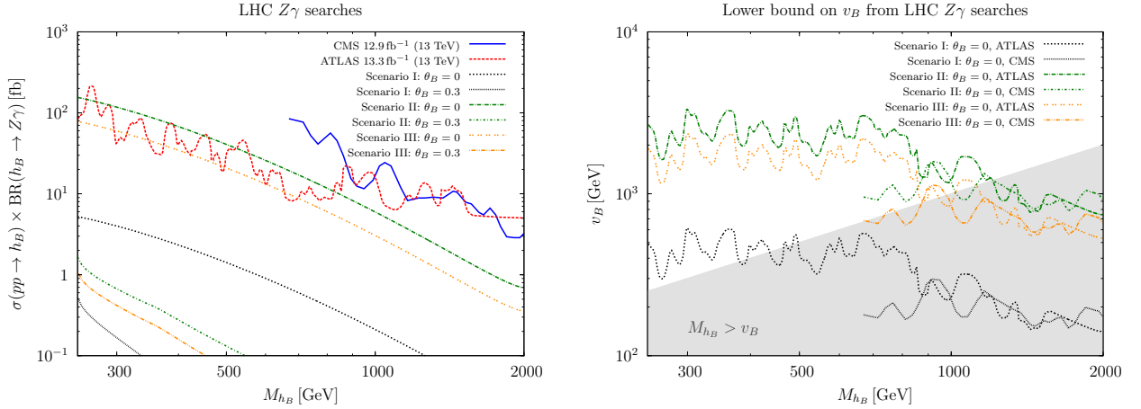
Figure 5. Constraints from Z\gamma searches [27, 28]. Left panel: experimental bounds as well as cross section predictions in scenarios I, II, and II as a function of the baryonic Higgs mass. Cross sections are shown both for negligible mixing angle and for a near maximal value of \theta_B = 0.3 . Right panel: experimental bounds translated into lower limits on v_B as a function of M_{h_B} for the case of negligible mixing. In the left panel we use v_B = 2 TeV, and in both panels n_f = 3 and m_Q = 1 TeV.
