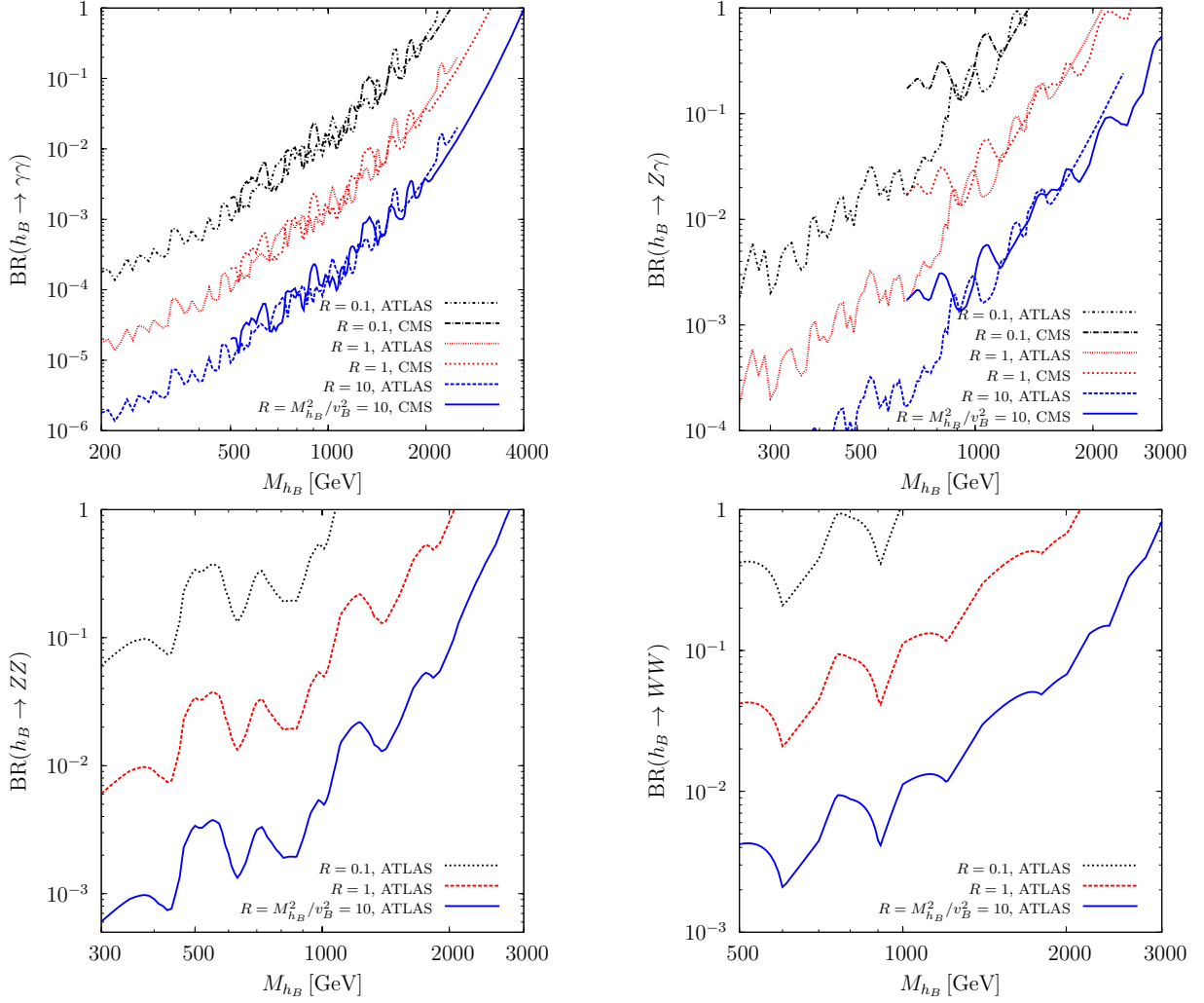
Figure 3. Constraints on the branching ratios of h_B into two photons [25, 26], Z\gamma [27, 28], ZZ [29], and WW [30] for different choices of the ratio between mass and vev of the baryonic Higgs field. In the plots n_f = 3 .
