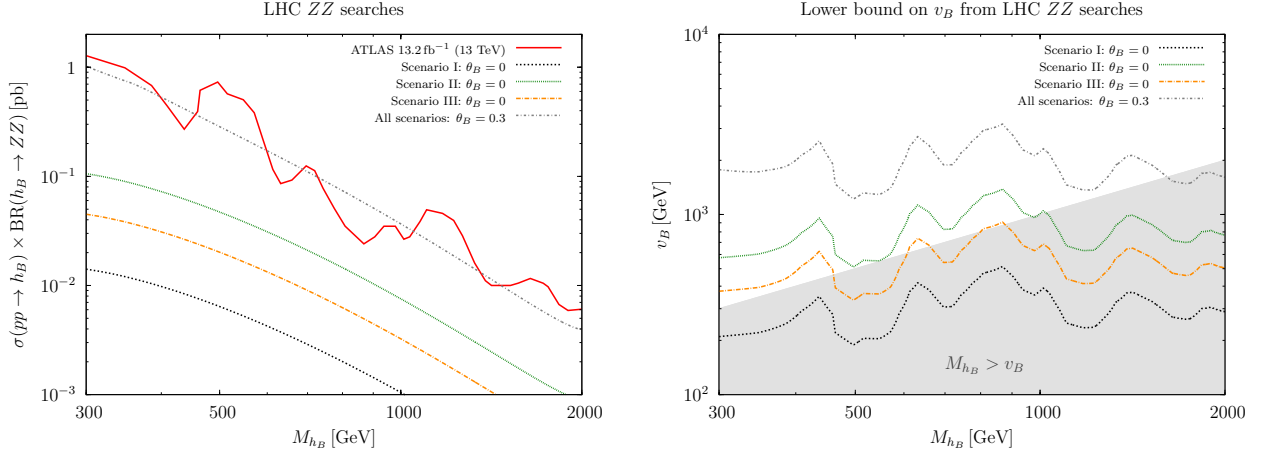
Figure 6. Constraints from ZZ searches [29]. Left panel: experimental bounds as well as cross section predictions in scenarios I, II, and II as a function of the baryonic Higgs mass. Cross sections are shown both for negligible mixing angle and for a near maximal value of \theta_B = 0.3 for which the three scenarios coincide. Right panel: experimental bounds translated into lower limits on v_B as a function of M_{h_B} . In the left panel we use v_B = 2 TeV, and in both panels n_f = 3 and m_Q = 1 TeV.
