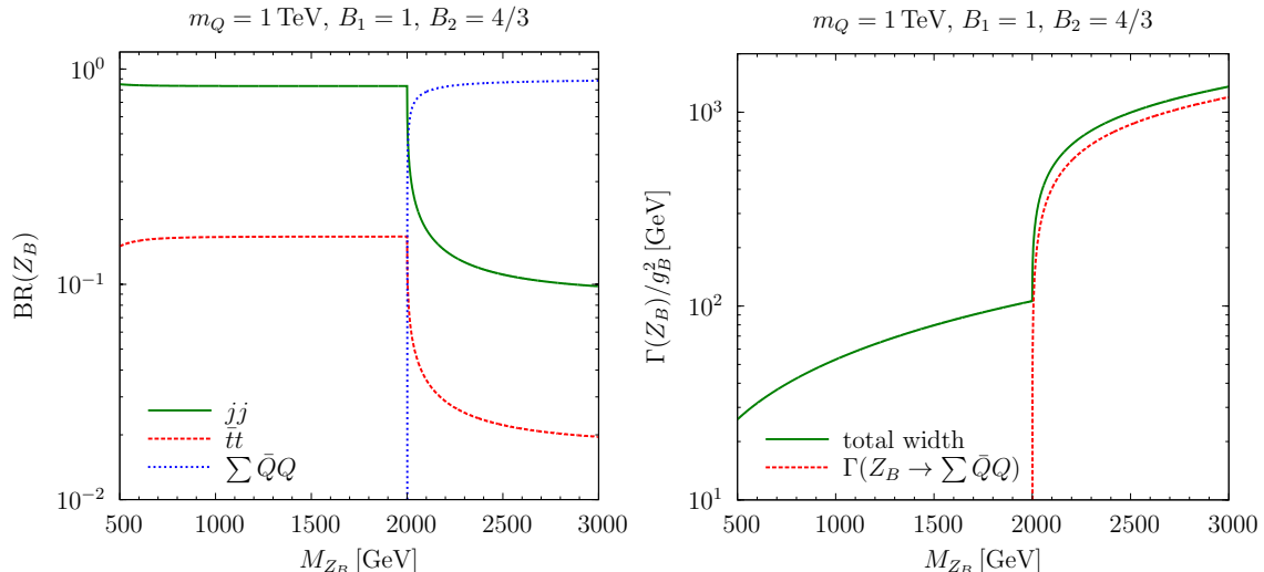
Figure 9. Branching ratios and total decay width of the leptophobic gauge boson. Here we assume m_Q = 1 TeV, B_1 = 1 and B_2 = 4/3 for illustration. The decays into all SM quarks except for the top quarks are included in the jj decays.
