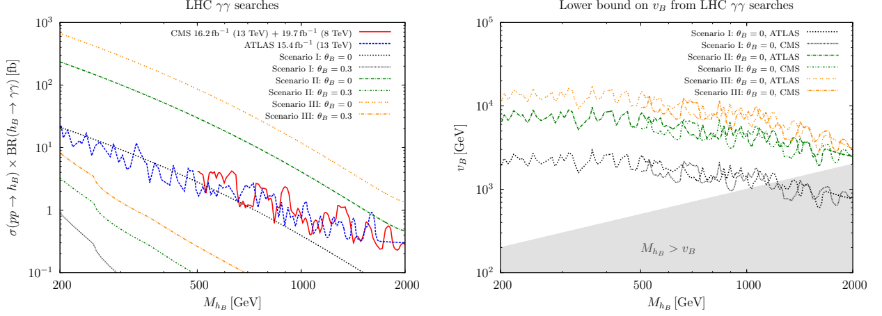
Figure 4. Constraints from diphoton searches [25, 26]. Left panel: experimental bounds as well as cross section predictions in scenarios I, II, and III as a function of the baryonic Higgs mass. Cross sections are shown both for negligible mixing angle and for a near maximal value of \theta_B = 0.3 . Right panel: experimental bounds translated into lower limits on v_B as a function of M_{h_B} for the case of negligible mixing. In the left panel we use v_B = 2 TeV, and in both panels n_f = 3 and m_Q = 1 TeV.
