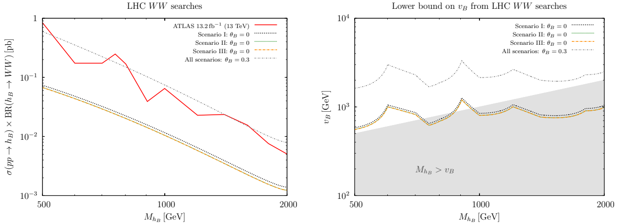
Figure 7. Constraints from WW searches [30]. Left panel: experimental bounds as well as cross section predictions in scenarios I, II, and II as a function of the baryonic Higgs mass. Cross sections are shown both for negligible mixing angle and for a near maximal value of \theta_B = 0.3 for which the three scenarios coincide. Right panel: experimental bounds translated into lower limits on v_B as a function of M_{h_B} . In the left panel we use v_B = 2 TeV, and in both panels n_f = 3 and m_Q = 1 TeV.
