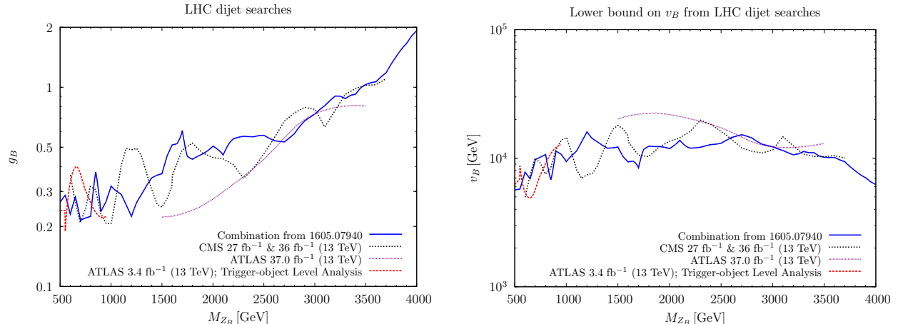
Figure 8. Current experimental constraints on leptophobic gauge bosons from dijet searches [31–34]. Left panel: upper bound on g_B as a function of M_{Z_B} . Right panel: re-interpretation of the bounds in the mass-coupling plane as a lower bound on the symmetry breaking scale v_B .
