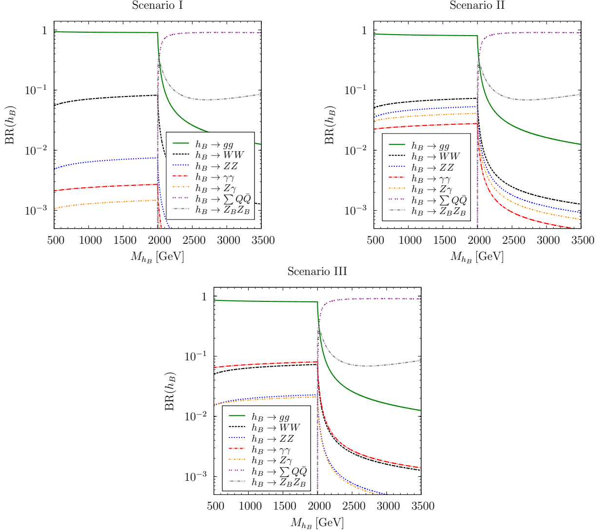
Figure 2. Branching ratios of the baryonic Higgs as a function of its mass M_{h_B} assuming negligible mixing angle \theta_B . We use M_{Z_B} = 1 TeV, v_B = 20 TeV and m_Q = 1 TeV.
