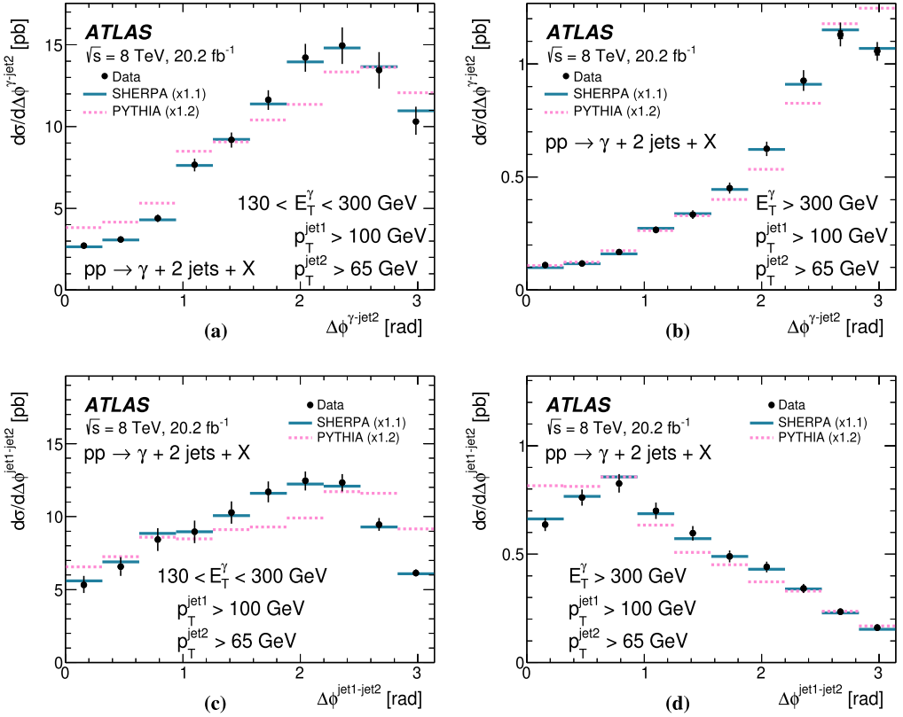
Fig. 11. Measured cross sections for isolated-photon plus two-jet production (dots) as functions of (a, b) \Delta\phi^{\gamma\text{-jet2}} and (c, d) \Delta\phi^{\text{jet1-jet2}} for (a, c) E_T^\gamma < 300 GeV and (b, d) E_T^\gamma > 300 GeV. For comparison, the predictions from PYTHIA (dashed lines) and SHERPA (solid lines) are also shown. The predictions are normalised to the data by a global factor, which is indicated in parentheses. The inner (outer) error bars represent the statistical uncertainties (the statistical and systematic uncertainties added in quadrature). For most of the points, the inner error bars are smaller than the marker size and, thus, not visible.
