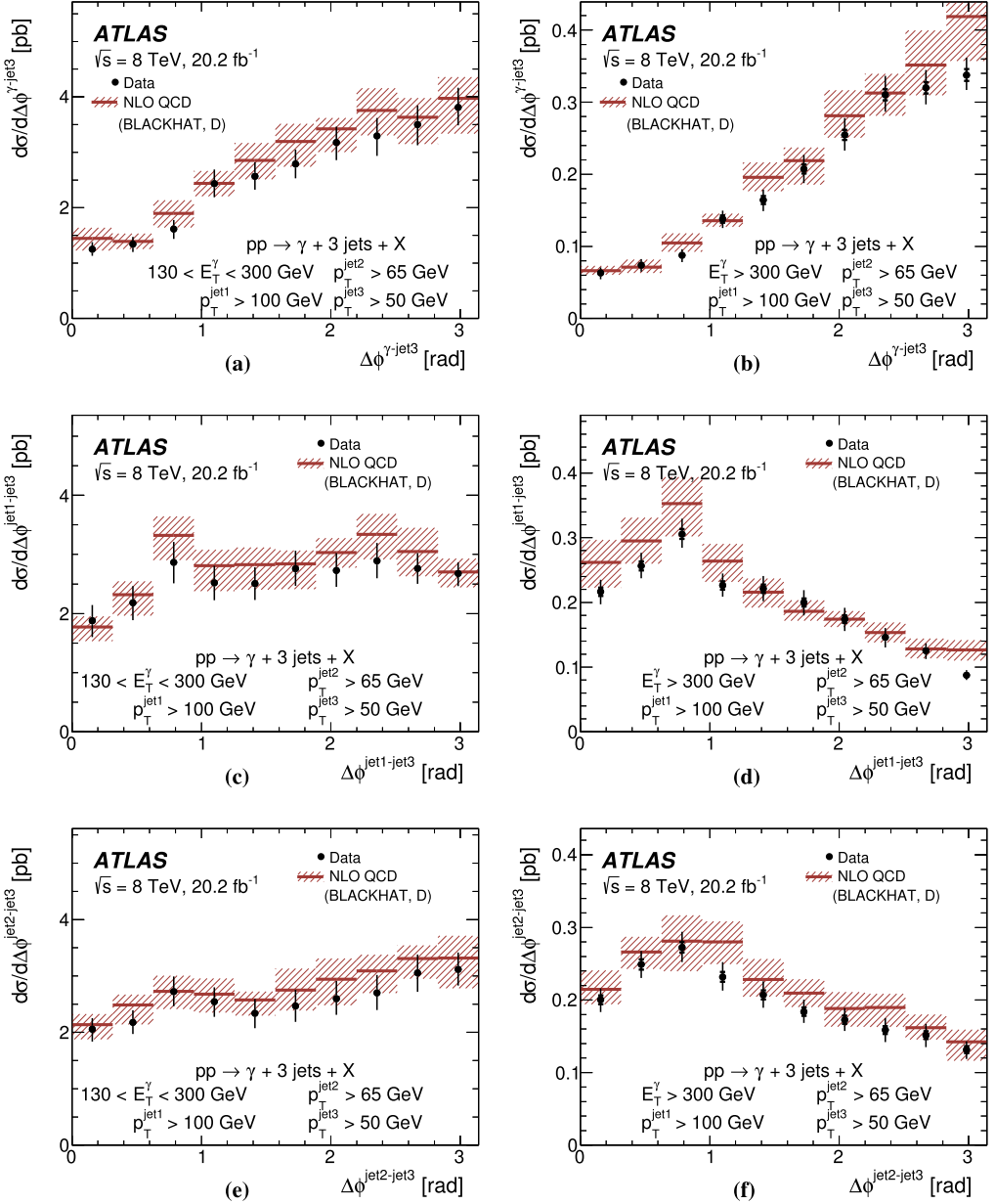
Fig. 15. Measured cross sections for isolated-photon plus three-jet production (dots) as functions of (a, b) \Delta\phi^{\gamma\text{-jet}3} , (c, d) \Delta\phi^{\text{jet}1\text{-jet}3} and (e, f) \Delta\phi^{\text{jet}2\text{-jet}3} for (a, c, e) E_T^\gamma < 300 \text{ GeV} and (b, d, f) E_T^\gamma > 300 \text{ GeV} . The NLO QCD predictions from BLACKHAT corrected for hadronisation and underlying-event effects and using the CT10 PDF set are also shown as solid lines. These predictions include only the direct contribution (D). The inner (outer) error bars represent the statistical uncertainties (the statistical and systematic uncertainties added in quadrature) and the shaded band represents the theoretical uncertainty. For most of the points, the inner error bars are smaller than the marker size and, thus, not visible.
