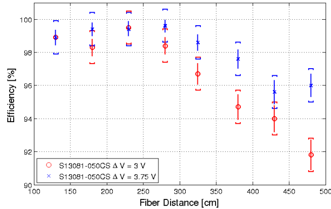
Figure 12. Efficiency measurements for two different \Delta V are compared. A larger \Delta V produces an increase in the efficiency. The estimated integrated efficiency is: 97 % for \Delta V = 3\text{ V} (red) and 98 % for \Delta V = 3.75\text{ V} (blue). Vertical lines represent statistic errors assuming a binomial distribution and brackets represent the systematics errors caused by false triggers.
