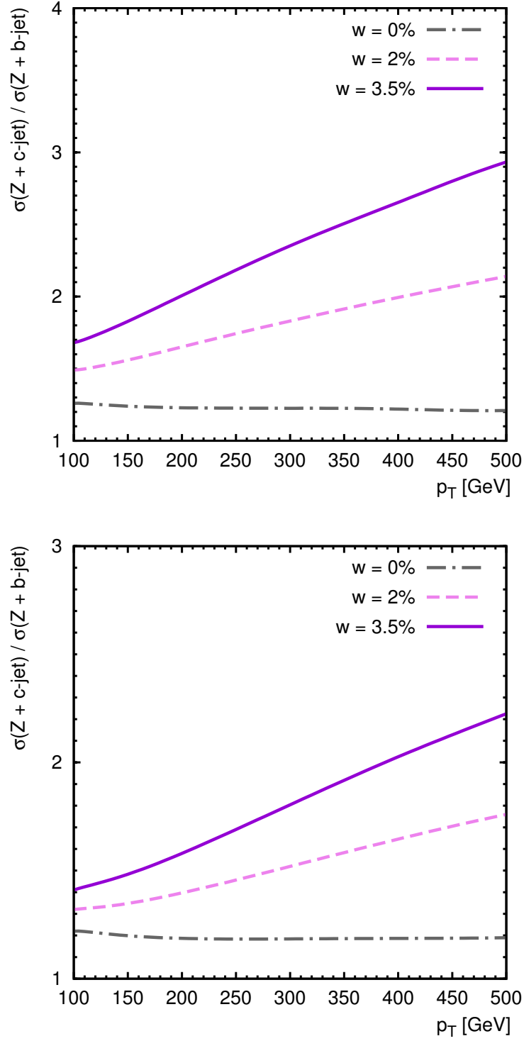
Figure 6: The cross section ratio of the Z + c production to the Z + b one in the pp collision calculated as a function of the Z boson transverse momentum p_T at \sqrt{s} = 8 TeV (top) and \sqrt{s} = 13 TeV (bottom) within the k_T -factorization approach. The kinematical conditions are described in the text.
