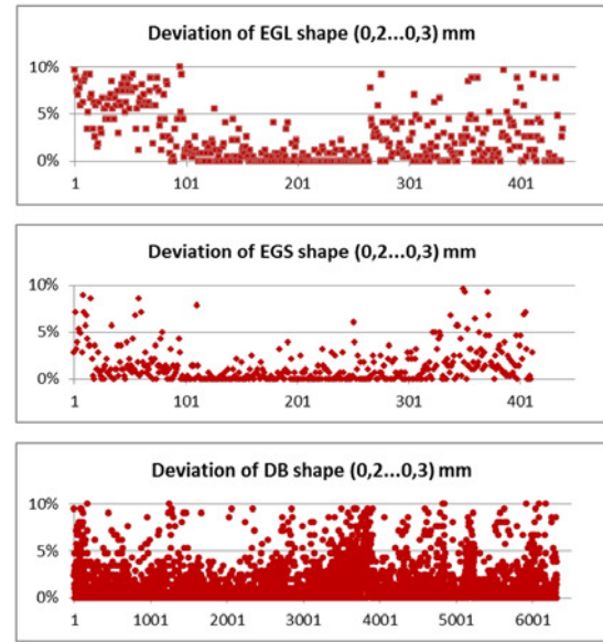
Figure 5: Part of subcomponents shape with accuracy deviation over 0.2 mm.
