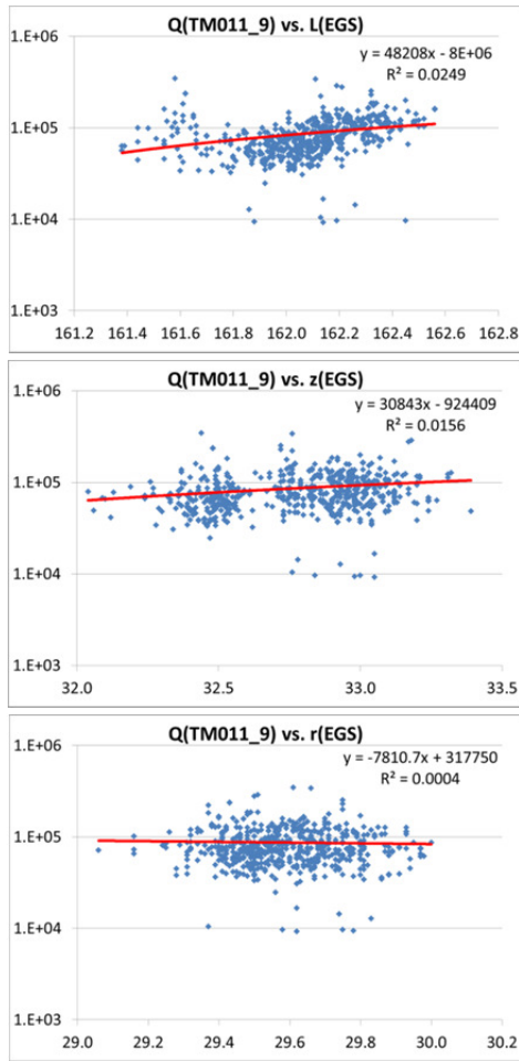
Figure 3: Sensitivities of quality factor for TM011 (y) to EGS geometry deviations (x = L, z and r) in mm.
