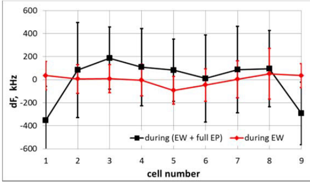
Figure 6: Calculated frequencies deviations in different cells during EW and EP.
