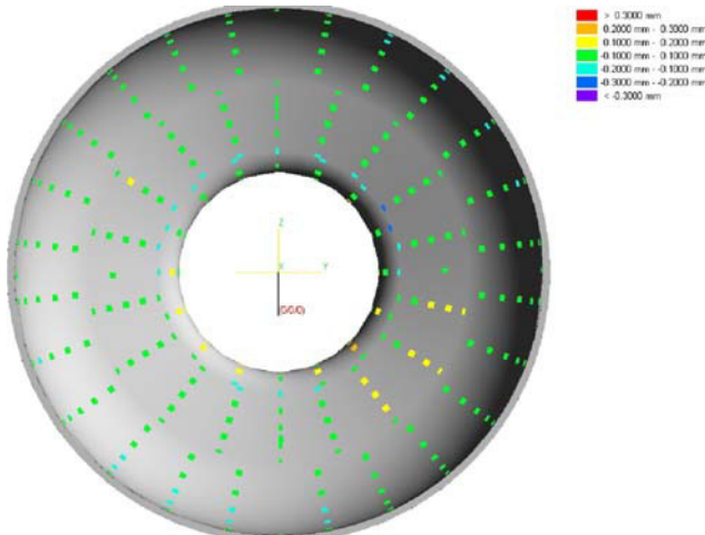
Figure 4: Results of 3D-measurements of cavity half-cell.
