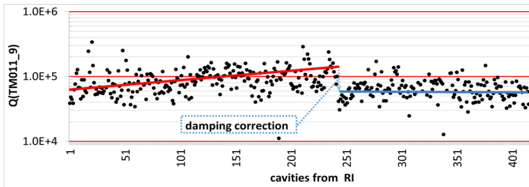
Figure 1: Measurements results of the Q_{load} for the TM011 (zero-mode) at 2K.
