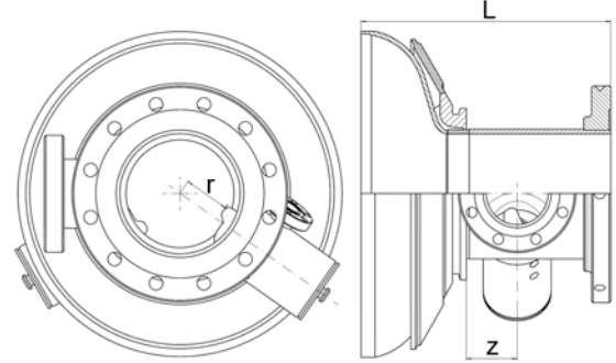
Figure 2: Position of the HOM coupler #1 in EGS: L – length; z – distance between coupler and connecting flange, r – distance between cavity axis and F-part.
