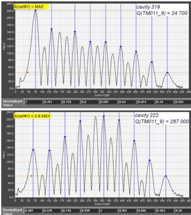
Figure 7: E-field distribution of the TM011_9 on axis for two examples: cavity 319 with asymmetrical field; cavity 222 with symmetrical “trapped” field.
