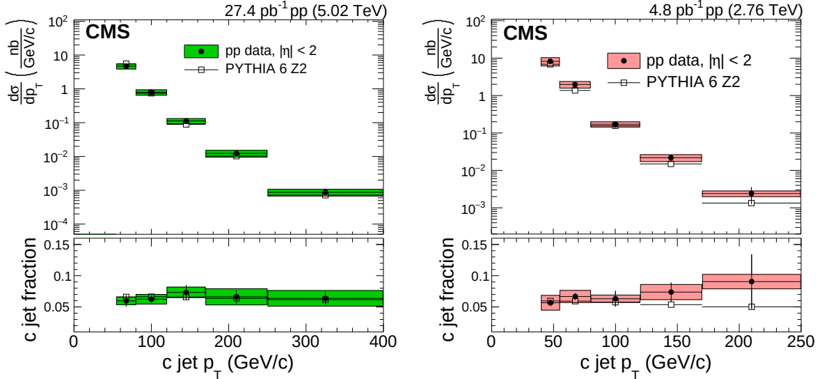
Figure 6: The c jet spectra (top) and fraction (bottom) as a function of c jet p_T for 5.02 TeV (left) and 2.76 TeV pp data (right), compared to predictions from PYTHIA 6. Systematic uncertainties are shown as filled boxes.
