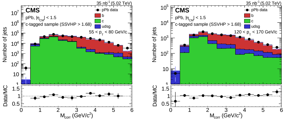
Figure 2: Corrected secondary vertex mass distributions from PYTHIA+HIJING for c jets (green), light parton jets (blue), and b jets (red) in the jet p_T range 55–80 \text{GeV}/c (left) and 120–170 \text{GeV}/c (right). Relative normalizations of these three distributions are fit to a distribution from pPb collision data (black). Statistical uncertainties are shown in black for data and for individual simulated flavor components and are shown in blue for the sum of the simulated distribution. The bottom panels of both plots show the ratio of data to simulation.
