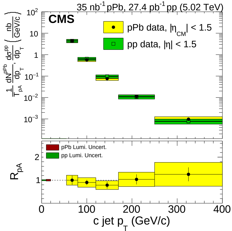
Figure 7: The c jet spectrum (top) and R_{pA} (bottom) as a function of c jet p_T for 5.02 TeV pPb and pp data. Statistical uncertainties are solid black lines, while systematic uncertainties are shown as filled colored boxes. Integrated luminosity uncertainties for pp and pPb data are shown as filled boxes around unity.
