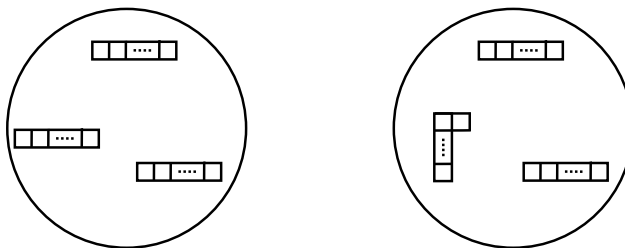
Figure 3. On the left we depict the sphere with three full punctures that corresponds to the un-Higgsed T_N with SU(N)^3 global symmetry. On the right we show the sphere with two full punctures and one L-shaped \{N-1, 1\} puncture. This particular Higgsing of T_N leads to a theory with SU(N) \times SU(N) \times U(1) global symmetry. The partition function of this theory will lead to the Toda 3-point function with one semi-degenerate primary insertion.
