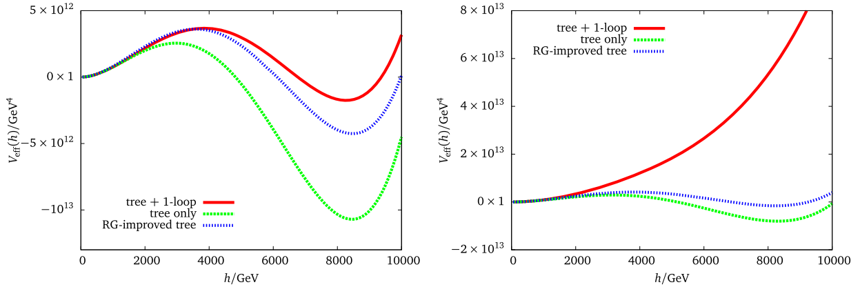
Fig. 3. For a given parameter point ( \mu = 4 TeV, \tan\beta = 40 , A_t = 1.8 TeV), we show exemplarily the behavior of the potential in the given direction in field space (and \tilde{b} = 0.75h_u^0 ). On the left-hand side, the positive sign for h_d^0 was chosen, where the plot on the right has h_d^0 = -\sqrt{|h_u^0|^2 + |\tilde{b}|^2} with real fields and parameters in both cases. The “tree + 1-loop” line means inclusion of the one-loop Higgs potential as of Eq. (2) plus the tree-level bottom squark potential (without D -terms each since they vanish by definition of the direction) evaluated with running parameters (soft-breaking squark masses and Yukawa couplings). For comparison, we show the “tree only” where the masses and couplings of the potential have been evaluated at the SUSY scale M_{\text{SUSY}} = 1 TeV and the “RG-improved tree” potential where all soft masses and couplings are treated as running ones.
