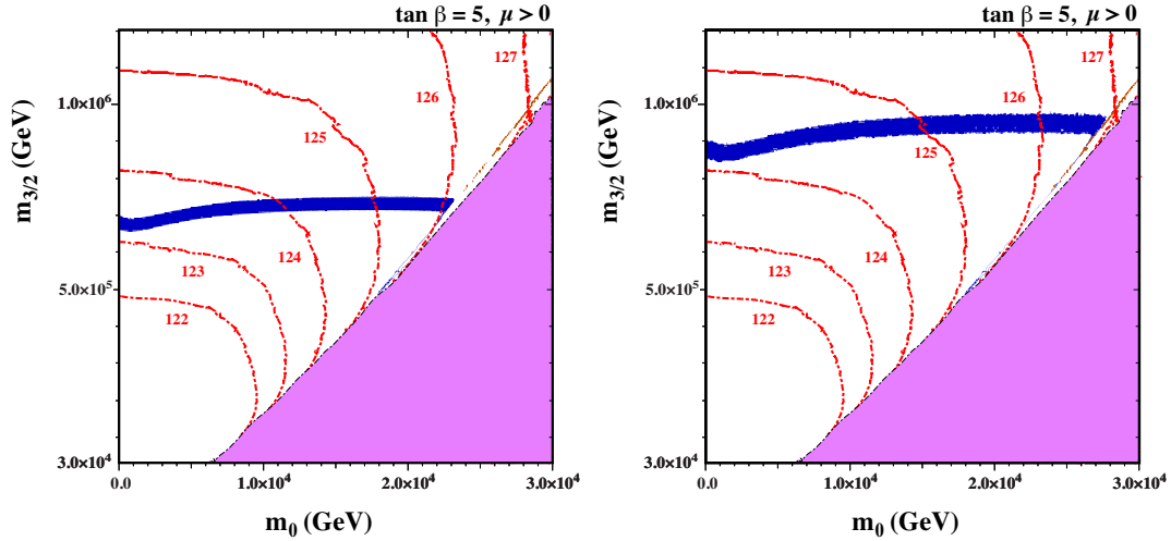
Figure 2. The (m_0, m_{3/2}) plane for \tan \beta = 5 without (left panel) and with (right panel) the Sommerfeld enhancement, as calculated using SSARD [36]. There are no consistent solutions of the electroweak vacuum conditions in the pink shaded triangular regions at lower right. The \tilde{\chi}_1^0 LSP density falls within the range of the CDM density indicated by Planck and other experiments in the dark blue shaded bands. Contours of M_h calculated using FeynHiggs 2.11.3 (see text) are shown as red dashed lines.
