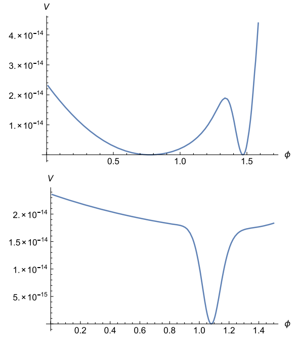
FIG. 4. The effective scalar potential for product separable models with tuned profile (31) (upper panel) and generic profile (33) (lower panel). Note the presence of the universal Minkowski minimum in both cases. In the tuned setup, there is an additional Minkowski minimum before the waterfall point. (Parameters are W_0 = -0.0004 , A = 1 , a = 0.1 , \alpha = 1 .)
