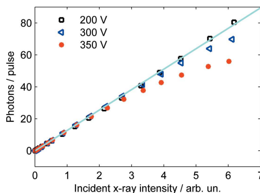
Figure 7 Mean APD signal as a function of incident X-ray intensity for 200 V, 300 V and 350 V APD bias voltages, derived from the histograms in Fig. 6. The APD signal is given in units of Fe fluorescence photons, which constitute mainly K_{\alpha} photons of 6.4 keV. At the highest bias of 350 V the APD response is linear up to a mean signal of 20 photons, at 300 V bias up to 40 photons and at 200 V bias of beyond 80 photons.
