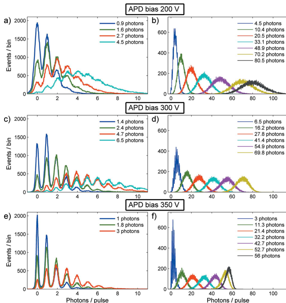
Figure 6 Integrated detector signal for a collection of single measurements (or pulse height distributions) for 200 V bias and low (a) and high (b) photon flux, 300 V bias with low (c) and high (d) photon flux, 350 V bias with low (e) and high (f) photon flux. The strong preamplifier gain amplifies the signal to its limiting value leading to the asymmetric pulse shape near 60 photons in (f) (see also Fig. 7).
