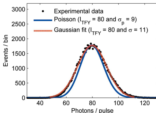
Figure 5 Pulse height distribution of the integrated APD single pulse intensity for 10^5 X-ray pulses (black dots). A mean flux of 80 photons per pulse is derived, when scaling the measured signal to the values as derived in Fig. 4. A Poisson function with I_{\text{TFY}} = 80 (blue solid line) and Gaussian fit to the data with \sigma = 11 (red dashed line) are shown for comparison.
