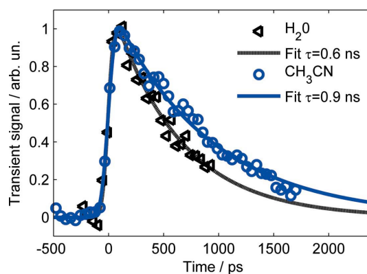
Figure 9 Time-delay scan of the transient signal of [\text{Fe}^{\text{II}}(\text{bpy})_3]^{2+} in \text{H}_2\text{O} (black triangles) and \text{CH}_3\text{CN} (blue circles) at 7125 eV (arrow in Fig. 8), together with a fit of a Gaussian error function convoluted with a single exponential decay. The decay times of 0.6 ns in \text{H}_2\text{O} (dotted black line) and 0.9 ns in \text{CH}_3\text{CN} (solid blue line) agree with the literature data. The rise time of 0.1 ns is almost equivalent to the pulse duration of the X-rays. The relatively low S/N of \sim 20 is due to the fact that these spectra were recorded with relatively poor laser/X-ray overlap conditions (after these initial time-delay scans we usually optimize overlap conditions to achieve S/N values as shown, for example, in Fig. 8).
