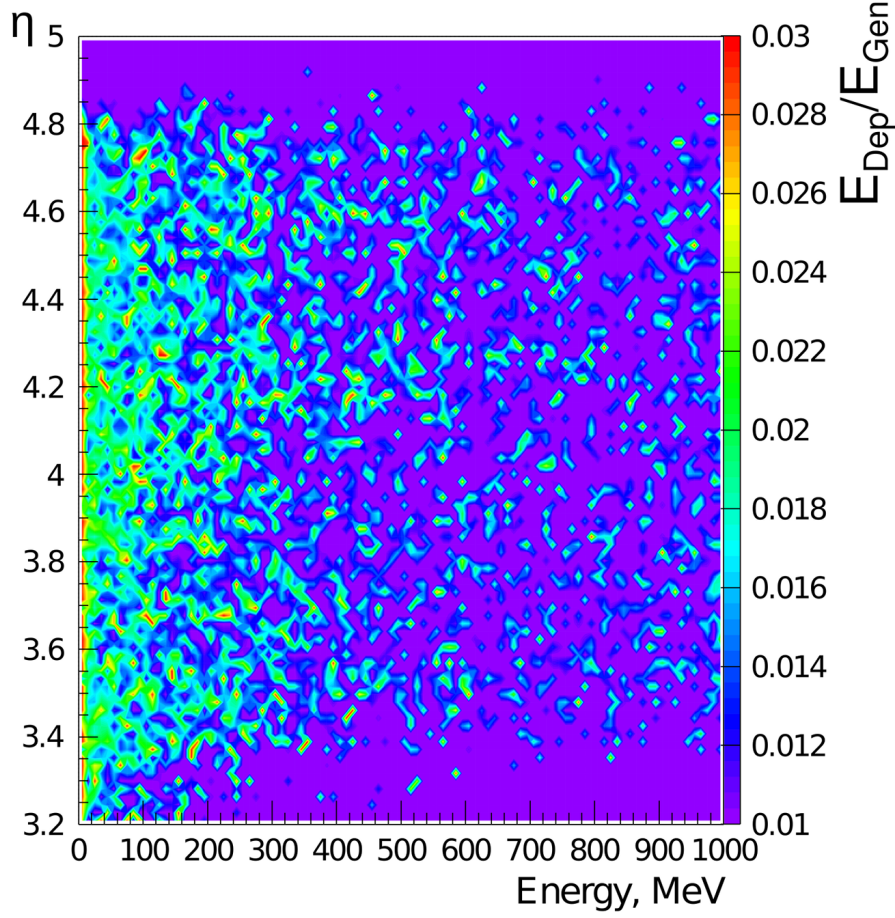
Figure 6.5: The diagram showing the population of the FCAL library for electrons over \eta -energy kinematic plane. The color scale shows not the density of the showers, but rather the energy response, i.e. the amount of energy registered by the calorimeter versus the initial energy of the starting point. The density of the showers can be derived from the amount of the purple zero-level, which means “no showers present in this region”. It can be seen that the average response of the calorimeter is about 2% and also that the lower-energy bins are much more populated than the higher-energy bins.
