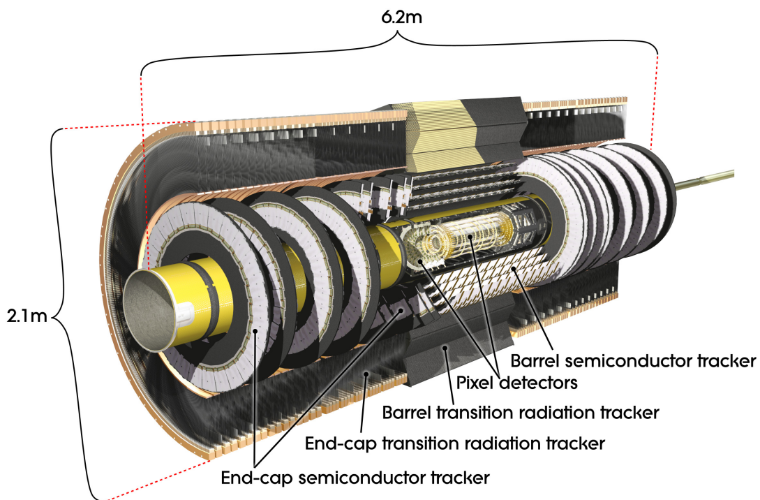
Figure 4.2: Overview of the ATLAS tracker. The SCT, TRT and pixel detectors are shown there. [78].
