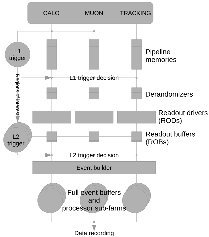
Figure 4.6: Diagram of the ATLAS trigger and readout system.
