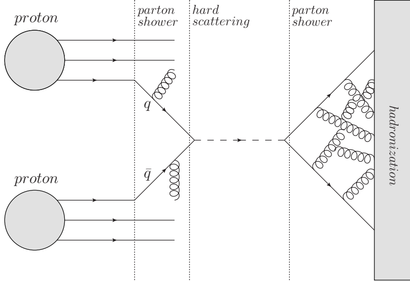
Figure 2.3: The deep inelastic scattering of two protons. The three main phases of the process are shown: initial radiation, the hard scattering itself, when the gauge boson is produced, and a final state radiation. If the gauge boson decayed into quarks, the hadronization process takes place in the end, when these quarks decay into color-neutral hadrons.
