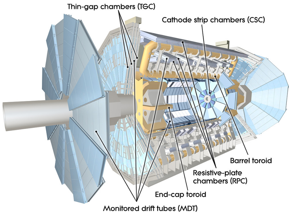
Figure 4.4: Overview of the ATLAS muon chambers. [78].
