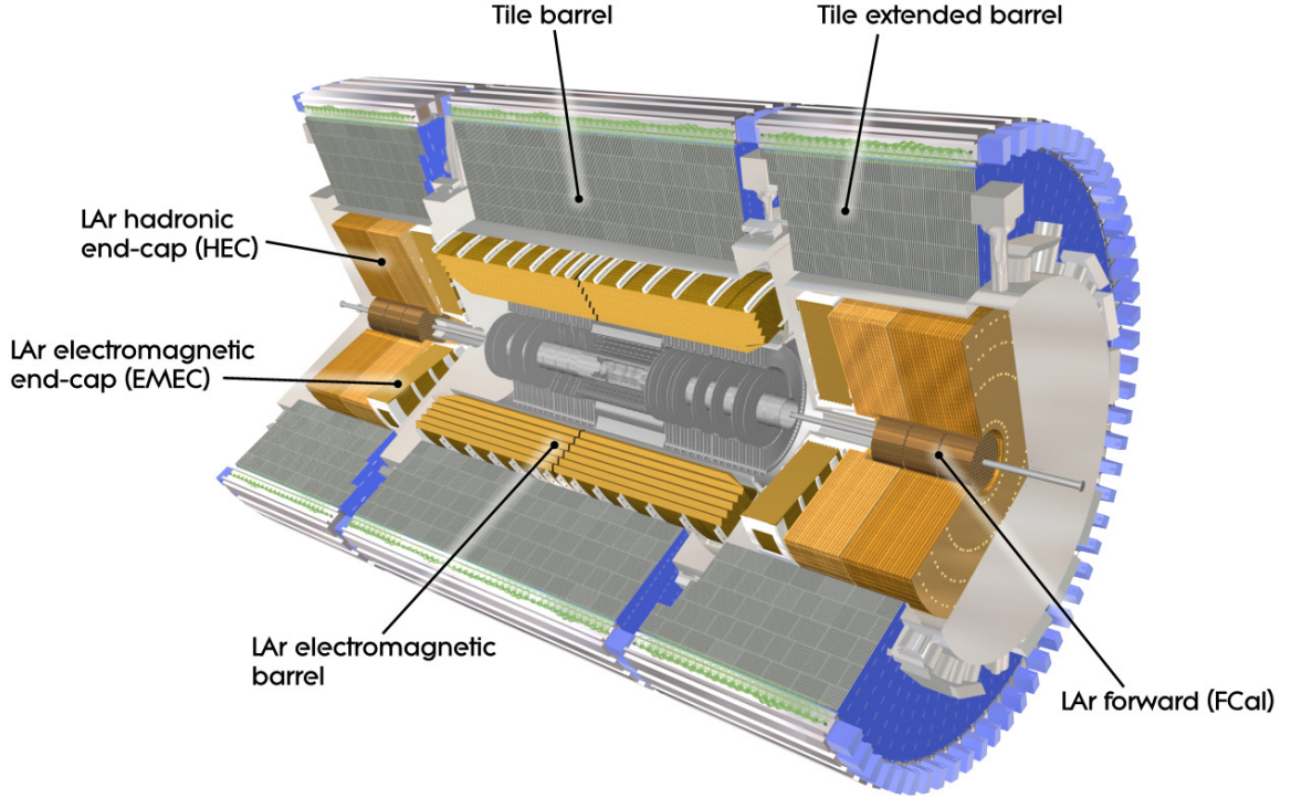
Figure 4.3: Overview of the ATLAS EM and hadronic calorimeters. [78].
