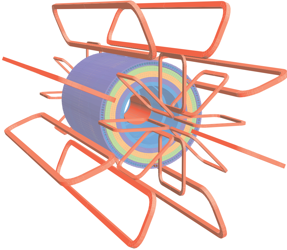
Figure 4.5: Overview of the ATLAS magnet system. [78].
