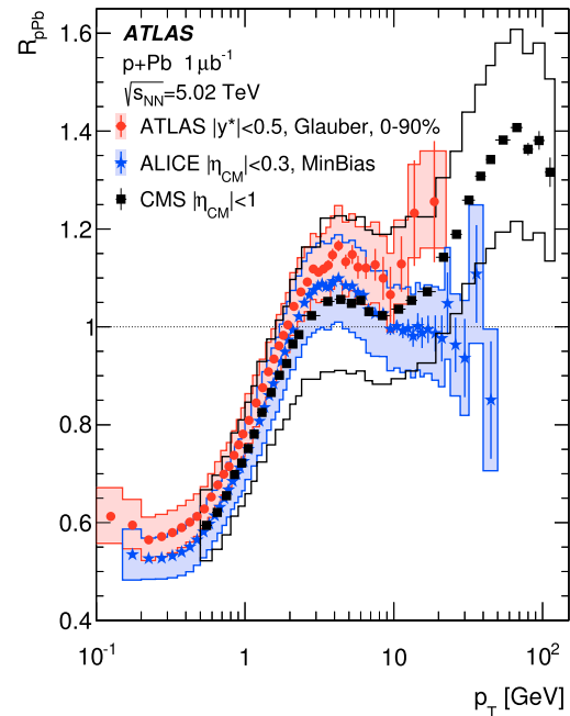
Fig. 6. R_{pPb} values as a function of p_T in the 0–90% centrality interval averaged over |y^*| < 0.5 , are compared to the minimum-bias (0–100%) results from a different pseudorapidity range in the centre-of-mass system: ALICE for |\eta_{CM}| < 0.3 [36] and CMS for |\eta_{CM}| < 1 [40]. The \langle T_{pB} \rangle value for the ATLAS centrality correction is calculated with the Glauber model. The total systematic uncertainties, which include the uncertainty in \langle T_{pB} \rangle , are indicated by lines of the same colour. Strict quantitative agreement is not expected as each measurement uses different rapidity intervals for the centrality determination and apply different event selection criteria to reject diffractive collisions.
