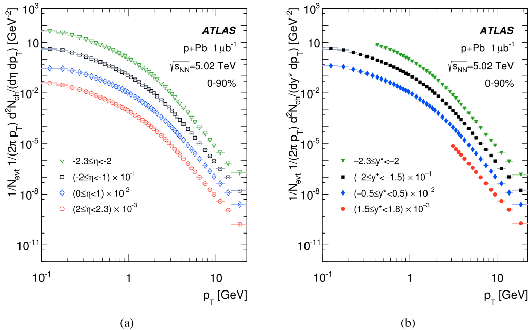
Fig. 3. Invariant differential p_T spectra of charged particles which are produced in p + \text{Pb} collisions at \sqrt{s} = 5.02 \text{ TeV} shown in (a) four \eta intervals and (b) four y^* intervals, for the 0–90% centrality interval. The individual spectra are scaled by constant factors (indicated in the legend) for visibility. The statistical uncertainties are indicated with vertical lines and the systematic uncertainties are indicated with boxes, but are generally much smaller than the size of the symbols.
