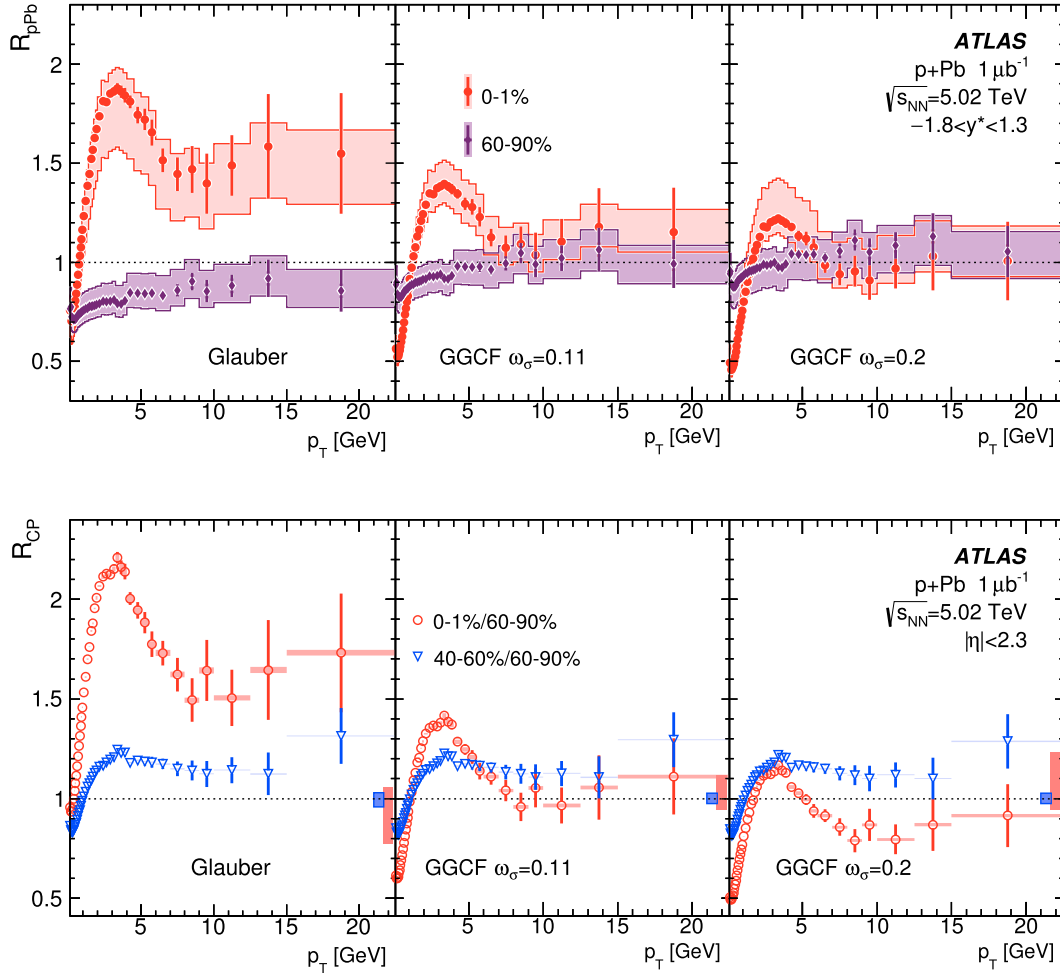
Fig. 7. (Top row) R_{pb} as a function of p_T extracted from the invariant yields integrated over -1.8 < y^* < 1.3 for the 0–1% and 60–90% centrality intervals, and for different geometrical models used to calculate \langle T_{pb} \rangle : Glauber, Glauber–Gribov \omega_\sigma = 0.11 and Glauber–Gribov \omega_\sigma = 0.2 ; (bottom row) R_{CP} for 0–1% and 40–60% central collisions with respect to the 60–90% centrality interval, also for the geometrical models, which are used to calculate \langle T_{pb} \rangle . Statistical errors are indicated with vertical lines and the systematic uncertainties in the invariant yields are indicated by a shaded area. The total systematic uncertainties, which include the uncertainty in \langle T_{pb} \rangle are indicated by lines of the same colour. The systematic uncertainties in the ratios of \langle T_{pb} \rangle are indicated by boxes of the same colour.
