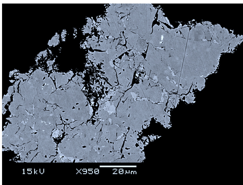
Fig. 4. Backscattered electron image of a recovered sample equilibrated at 17.5 GPa and 1223 K for 25 h and containing both the \epsilon -FeSi (brighter) and distorted-CuTi (darker) structures.
