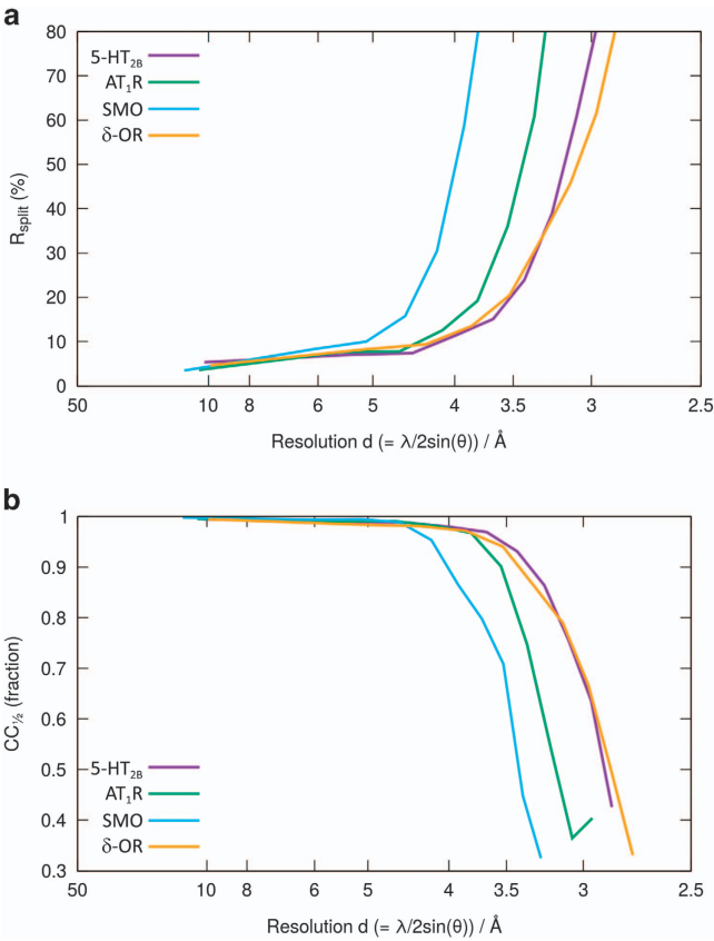
Figure 3. Plots of the self-consistency figures of merit (a) R_{\text{split}} and (b) CC_{1/2} against resolution for all four datasets as re-processed here.
