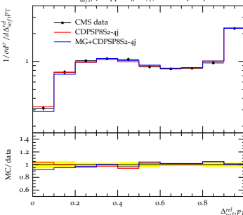
Normalized \Delta_{soft}^{rel} p_T in pp \rightarrow 4j in |\eta| < 4.7 at \sqrt{s} = 7 TeV
