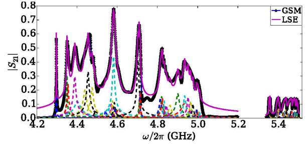
Figure 5: Fitting Lorentzian functions to S_{21} curves.
