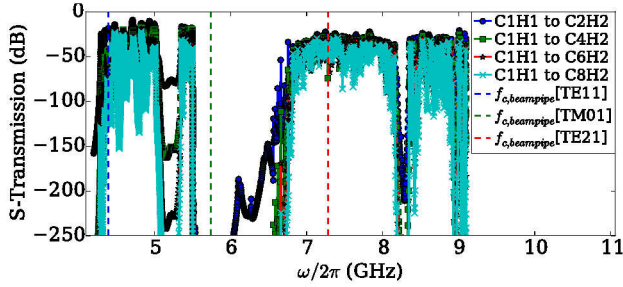
Figure 4: Amplitude of transmission coefficient along cavity chain.
