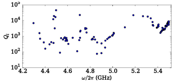
Figure 6: Q_l as a function of resonant frequency.
