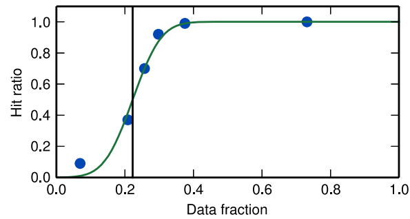
Figure 2. Determination of the threshold for hit finding. Diffraction patterns were sorted according to their number of ‘lit’ pixels in increasing order. Blue data points indicate the manually determined hit ratio for a sequence of 100 consecutive patterns in the sorted array. An error function (green line) approximates the data points. We define the hit threshold (black vertical line) at its inflection point. This corresponds to 400 ‘lit’ pixels and an overall hit ratio of 79%.
