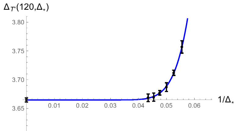
Figure 14. Extrapolation fit to determine the scaling dimension of the operator T' in the O(2) model with N = 120 points at \Delta_* = \infty from the results for that scaling dimension for different values of \Delta_* . The vertical error bar associated with the extrapolated point on the left corresponds to 1\sigma (68% confidence level).
