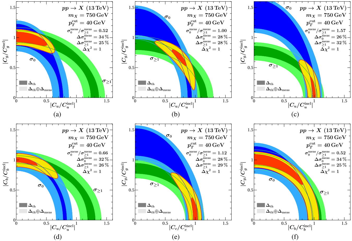
FIG. 2. \Delta\chi^2 = 1 -contours for various scenarios. (a) gluon signal, (b) mixed gluon/u-quark signal, (c) u -quark signal, (d) b -quark signal, (e) c -quark signal, (f) gluon signal. The constraints from \sigma_0 and \sigma_{\geq 1} are shown by the blue and green bands, respectively. The combined constraint from both are shown by the orange/yellow regions. The inner darker regions correspond to theory uncertainties only, while the full lighter bands include both theory and assumed experimental uncertainties.
