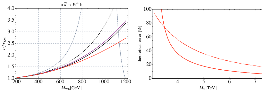
Figure 1. Left: the partonic u\bar{d} \rightarrow W^+h cross section as a function of the center-of-mass energy of the parton collision. The black lines correspond to the \text{SU}(2)_L triplet model with M_V = 1 TeV, g_H = -g_q = 0.25 (dashed), M_V = 2 TeV, g_H = -g_q = 0.5 (dotted), and M_V = 7 TeV, and g_H = -g_q = 1.75 (solid). The corresponding EFT predictions are shown in the linear approximation (solid red), and when quadratic terms in D=6 parameters are included in the calculation of the cross section (solid purple). Right: theory error as a function of M_V (solid line). The error is defined to be the relative difference between the constraints on g_*^2 \equiv g_H^2 = g_q^2 obtained by recasting the limits derived in the framework of a D=6 EFT and those derived from the resonance model. The limits come from re-interpreting the hypothetical experimental constraints with M_{\text{cut}} = 3 TeV, as described in the text. The dotted line corresponds to the naive estimate (M_{\text{cut}}/M_V)^2 .
