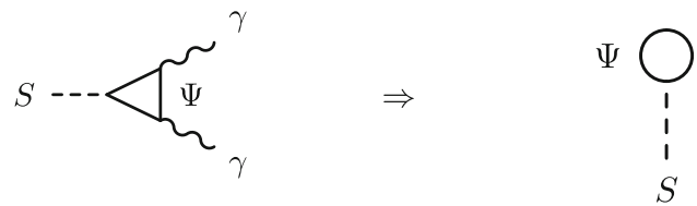
Fig. 5 Tadpole terms for S generated at one-loop level
