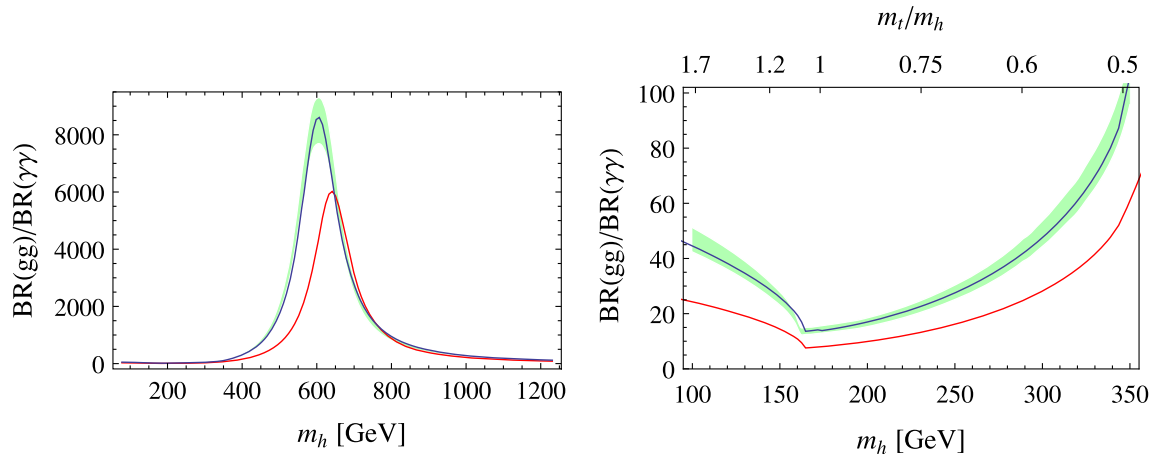
Fig. 9 \text{Br}(h \rightarrow gg)/\text{Br}(h \rightarrow \gamma\gamma) as calculated by SPheno at LO (red) and including higher order corrections as described in the text. The green band shows the values of the Higgs cross section working group including a 10 % uncertainty. On the right we zoom into the range m_h \in [0.5, 2] m_t
