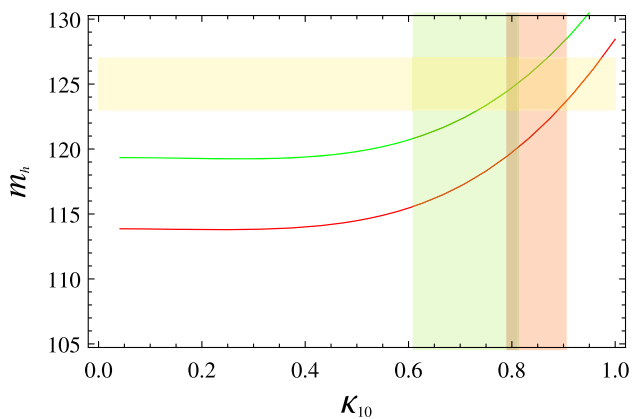
Fig. 6 Comparison of the two-loop Higgs mass calculation of Ref. [180] with the results obtained by SPheno. The parameters are those of Fig. 7 in Ref. [180] and we fixed X_{\kappa_{10}} = 0 . The lines are the results from SPheno, while the green and red shades areas are the ranges of \kappa_{10} which predict m_h = [123, 127] GeV according to Ref. [180]. Red takes X_t = 4 and green X_t = 2 , where X_t is defined in Eq. (9) of the reference
