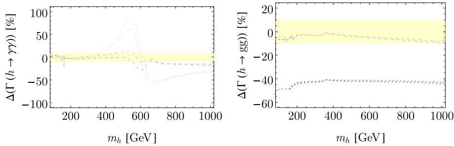
Fig. 8 On the left comparison of the relative difference in the partial width \Gamma(h \rightarrow \gamma\gamma) as calculated by SPheno (in red) and FlexibleSUSY (in blue) to the benchmark values provided by the Higgs cross section working group. The LO results are shown by the
