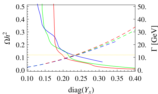
Fig. 24 Dark matter relic density \Omega h^2 (solid lines) of the lightest sneutrino and total width of the 750 GeV scalar (dashed lines) as function of Y_x . For the green line the relation Eq. (5.44) was used, while the red and blue lines deviate from this relation by \pm 0.4\% . The yellow shaded region is the 3\sigma band of Planck + WP + hihgL + BAO [476]
