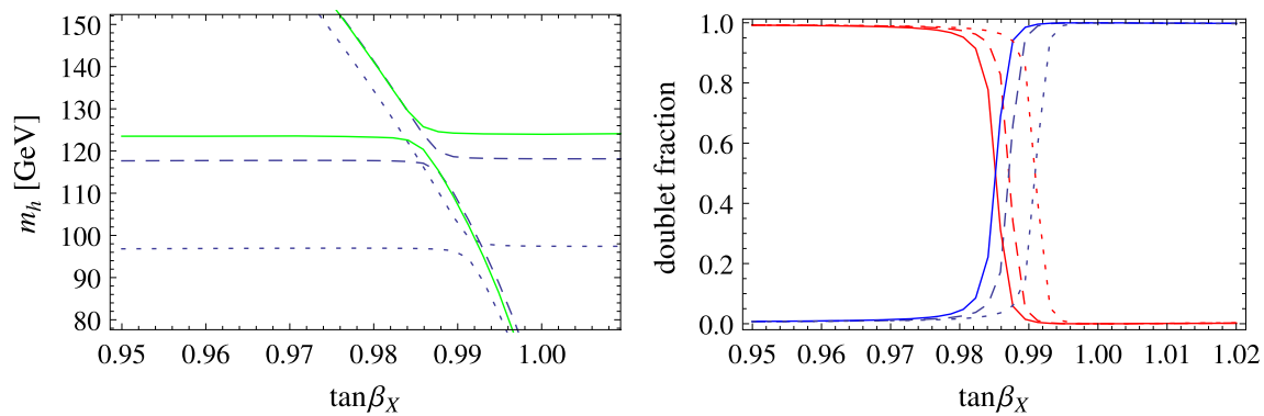
Fig. 21 Left the masses of the two lightest CP-even eigenstates as a function of \tan\beta_X at tree-level (dotted), one-loop (dashed) and two-loop (full green line). Right the corresponding doublet fraction of the
