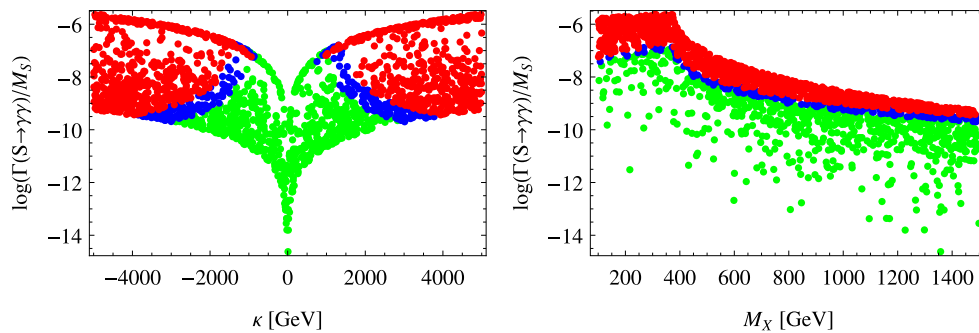
Fig. 2 \Gamma(S \rightarrow \gamma\gamma)/M_S as a function of \kappa (left) and M_X (right). Green points have a stable vacuum, blue points have a meta-stable but long-lived vacuum, while for the red ones it decays in a short time,
