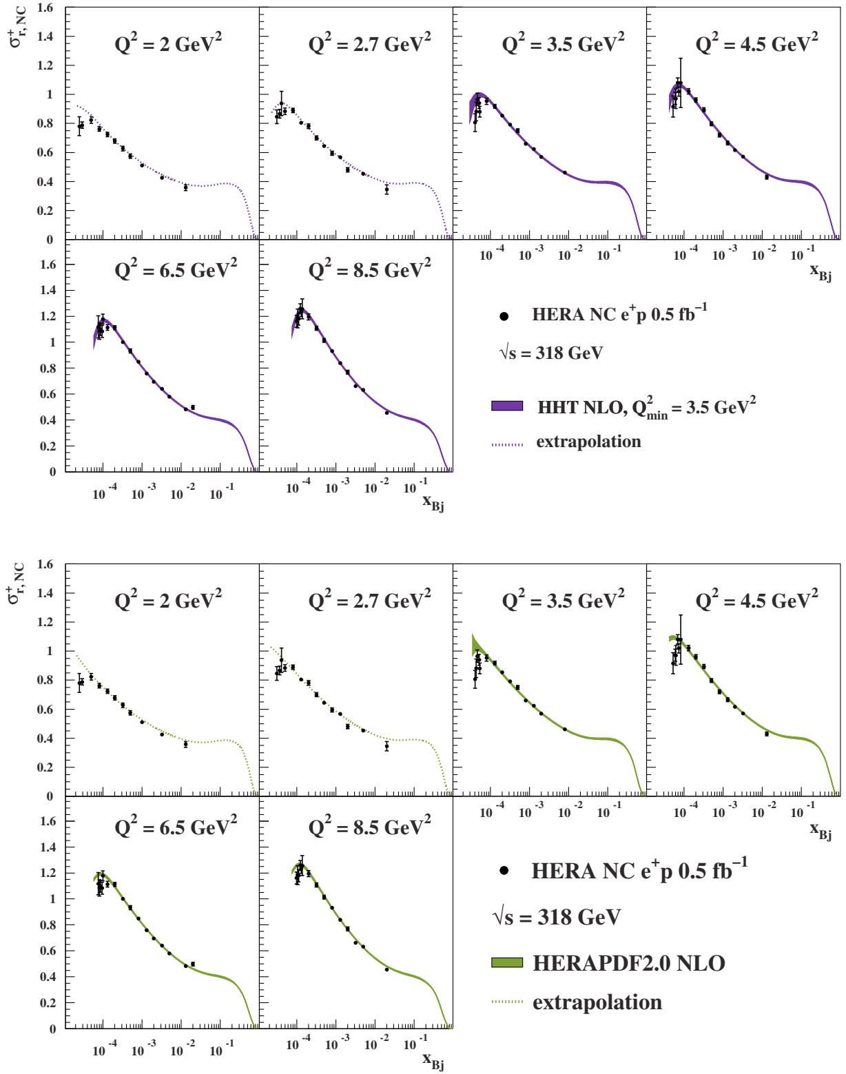
FIG. 5. The predictions of HHT NLO (top) and HERAPDF2.0 NLO (bottom), both with Q_{\min}^2 = 3.5 \text{ GeV}^2 , compared to the HERA measurements of \sigma_r^+ . The bands represent the experimental, i.e. fit, uncertainties. Extrapolations are indicated as dotted lines.
