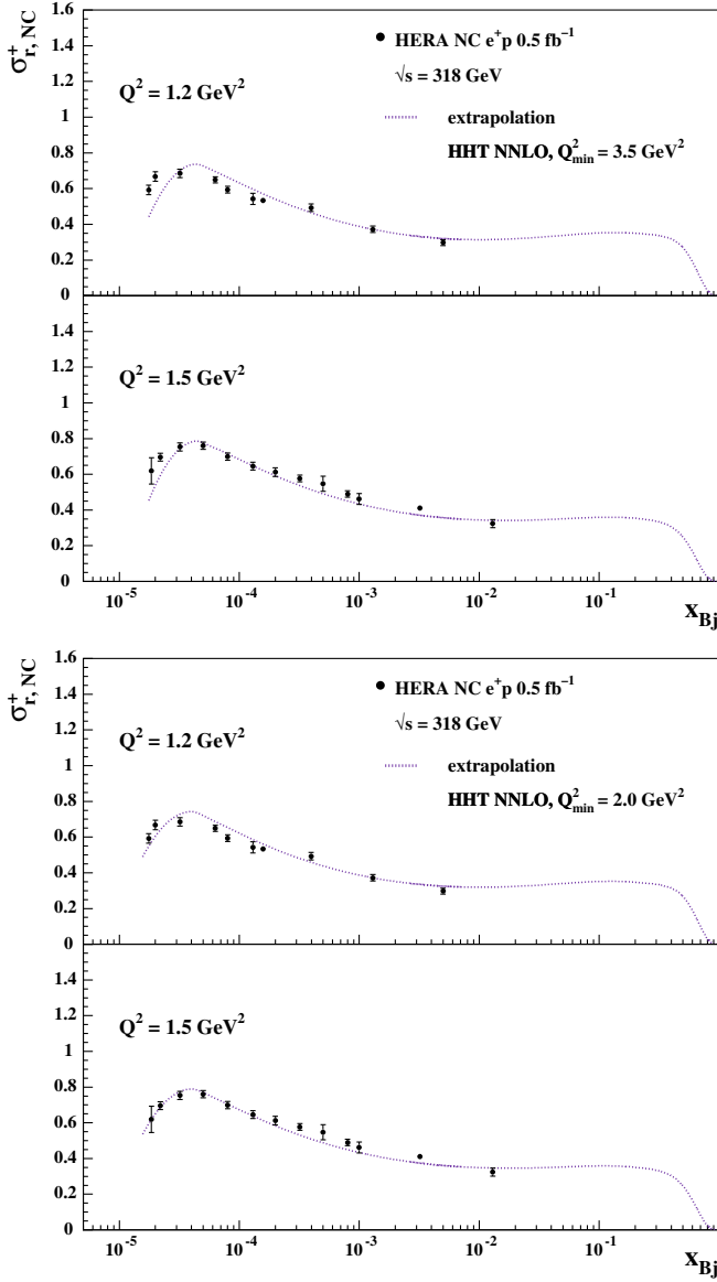
FIG. 7. The extrapolated predictions of HHT NNLO with Q^2_{\min} = 3.5 \text{ GeV}^2 (top) and with Q^2_{\min} = 2.0 \text{ GeV}^2 (bottom) compared to the HERA NC e^+p measurements of \sigma_r at Q^2 of 1.2 and 1.5 \text{GeV}^2 .
