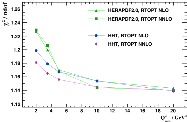
FIG. 2. The \chi^2/\text{ndof} versus Q_{\min}^2 for HHT and HERAPDF2.0 fits at NNLO and NLO.
