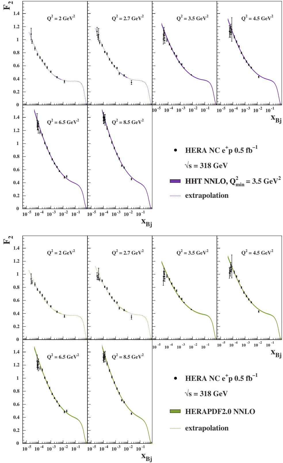
FIG. 8. The predictions of HHT NNLO (top) and HERAPDF2.0 NNLO (bottom), both with Q_{\min}^2 = 3.5 \text{ GeV}^2 , compared to extracted values F_2^{\text{extracted}} . The bands represent the experimental, i.e. fit, uncertainties. Extrapolations are indicated as dotted lines.
