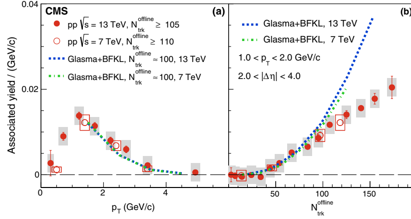
FIG. 3. Associated yield for the near side of the correlation function averaged over 2 < |\Delta\eta| < 4 and integrated over the region |\Delta\phi| < \Delta\phi_{\text{ZYAM}} for pp data at \sqrt{s} = 13 TeV (filled circles) and 7 TeV (open circles). Panel (a) shows the associated yield as a function of p_T for events with N_{\text{trk}}^{\text{off-line}} \geq 105 . The p_T value for each p_T bin is the average p_T value. In panel (b) the associated yield for 1 < p_T < 2 GeV/c is shown as a function of the multiplicity, N_{\text{trk}}^{\text{off-line}} . The N_{\text{trk}}^{\text{off-line}} value at which the yield is plotted is the average N_{\text{trk}}^{\text{off-line}} value in the bin. The p_T selection applies to both particles in each pair. The error bars correspond to the statistical uncertainties, while the shaded areas and boxes denote the systematic uncertainties. Curves represent the predictions of the gluon saturation model [39].
