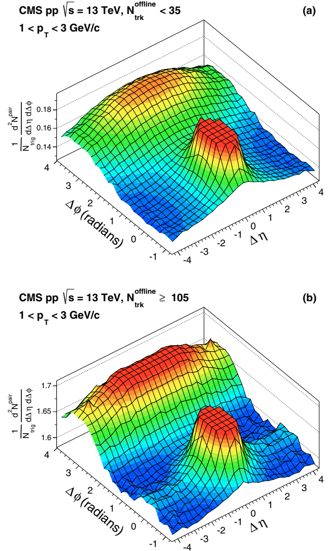
FIG. 1. The 2D (\Delta\eta, \Delta\phi) two-particle correlation functions in pp collisions at \sqrt{s} = 13 TeV for pairs of charged particles both in the range 1 < p_T < 3 GeV/c. Results are shown for (a) low-multiplicity events ( N_{\text{trk}}^{\text{off-line}} < 35 ) and for (b) a high-multiplicity sample ( N_{\text{trk}}^{\text{off-line}} \geq 105 ). The sharp peaks from jet correlations around (\Delta\eta, \Delta\phi) = (0,0) are truncated to better illustrate the long-range correlations.
