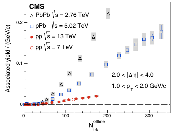
FIG. 4. Associated yield of long-range near-side two-particle correlations for 1 < p_T < 2 GeV/c in pp collisions at \sqrt{s} = 13 and 7 TeV, pPb collisions at \sqrt{s_{NN}} = 5.02 TeV, and PbPb collisions at \sqrt{s_{NN}} = 2.76 TeV. Associated yield for the near side of the correlation function is averaged over 2 < |\Delta\eta| < 4 and integrated over the region |\Delta\phi| < \Delta\phi_{\text{ZYAM}} . The N_{\text{trk}}^{\text{off-line}} value for each N_{\text{trk}}^{\text{off-line}} bin is the average N_{\text{trk}}^{\text{off-line}} value. The error bars correspond to the statistical uncertainties, while the shaded areas denote the systematic uncertainties. Note that there are PbPb points above the upper vertical scale, which are not shown for clarity.
