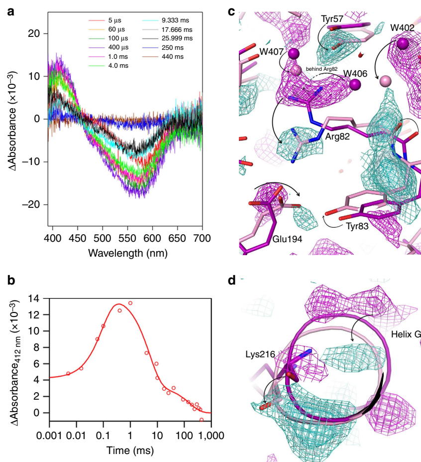
Figure 4 | Time-resolved absorption spectroscopy and crystallography on bR crystals. Time-resolved absorption spectroscopy on bR crystals ( a ) indicates similar photocycle kinetics as observed in purple membranes 44,58 . Absorption changes at 412 nm ( b ) indicate maximum accumulation of the M intermediate at ~1 ms after photoexcitation. The TR-SFX Fourier difference map with 1 ms time delay ( F_{\text{obs}}(\text{bR1ms}) - F_{\text{obs}}(\text{dark\_bR}) ; turquoise positive, magenta negative, shades represent 2.0, 2.5 and 3.0 \sigma ) is compatible with known light-induced conformational changes characteristic for the bR M intermediate (dark (purple), M state (pink) and 1CWQ 49 ). Reorganization in the proton transfer chain in the M intermediate involves a rotamer change of Arg82 and relocation of water molecules ( c ). Difference peaks around the site of retinal attachment Lys216 show a shift of helix G ( d ). Arrows indicate conformational changes apparent in the difference Fourier analysis.
